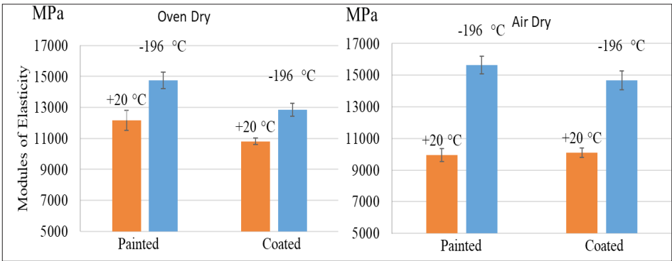
Figure 4: The effect of ultra-low temperature on the modules of elasticity of the painted and film-coated plywood.
