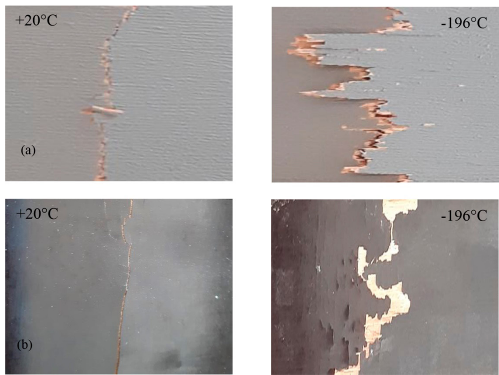
Figure 2: (a) Fracture characteristics of painted and (b) film-coated plywood between room temperature (+20 °C) and ultra-low temperature (-196 °C).
