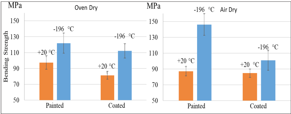
Figure 3: The effect of ultra-low temperature on the bending strength of the painted and film-coated plywood.
