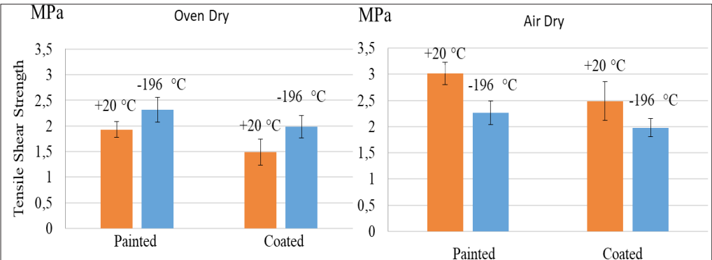
Figure 5: The effect of ultra-low temperature on the tensile shear strength of the painted and film-coated plywood.
