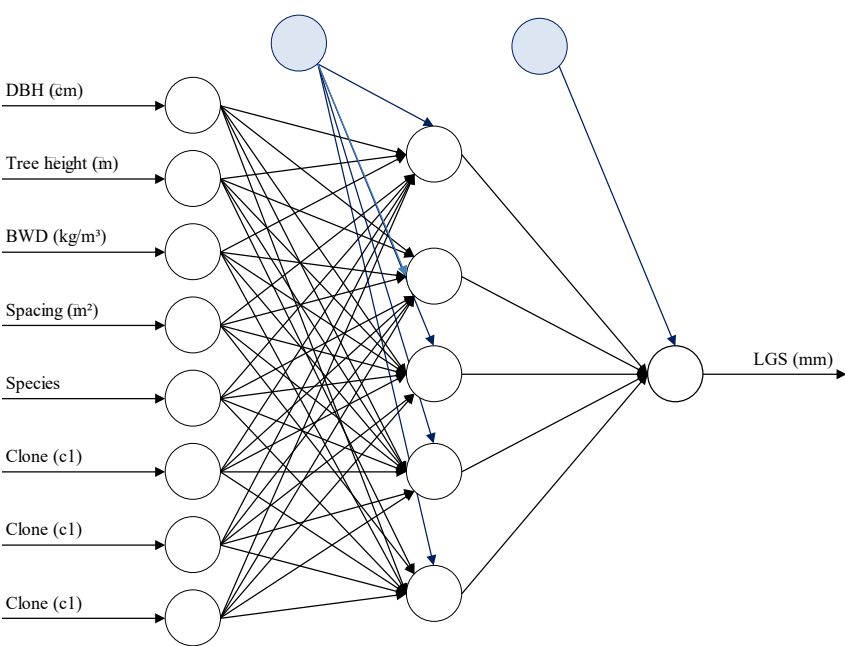
Figure 1: Artificial neural network structure model to estimate longitudinal growth strain with eight input neurons, five hidden neurons, and one output neuron.
