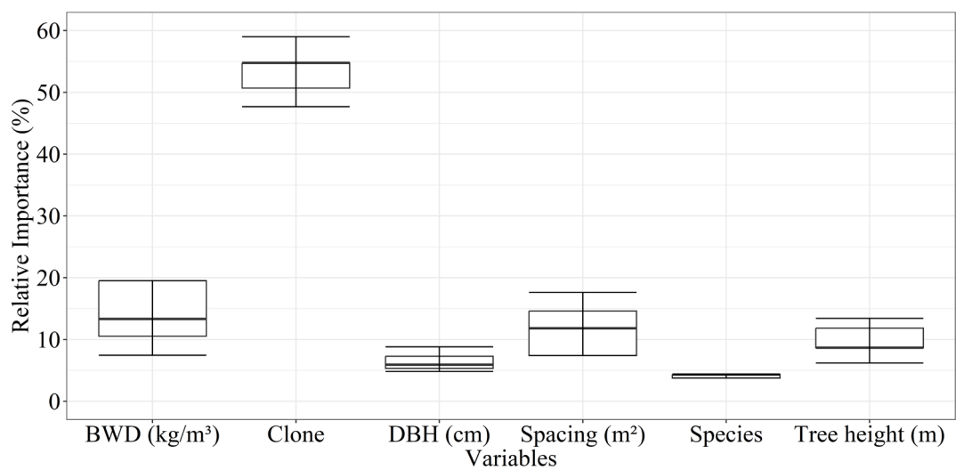
Figure 3: Boxplot for relative importance of artificial neural network input variables. Where: DBH = diameter at breast height; BWD = basic wood density; and LGS = longitudinal growth strain.
