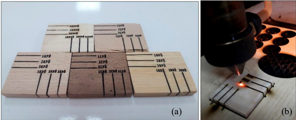
Figure 1: (a) Experiment samples, (b) laser cutting.
