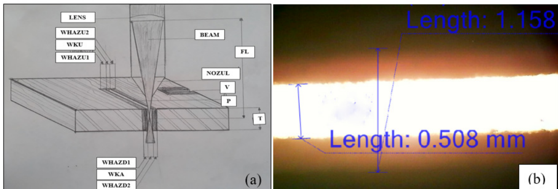
Figure 2: (a) The experimental setup Laser cuttings, (b) measurement method.
