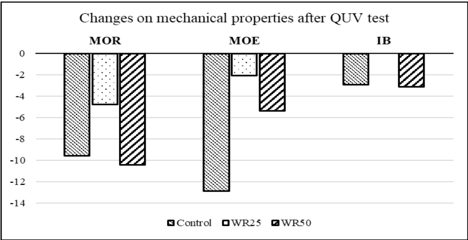
Figure 1: Changes on the mechanical properties after accelerated weathering test.
