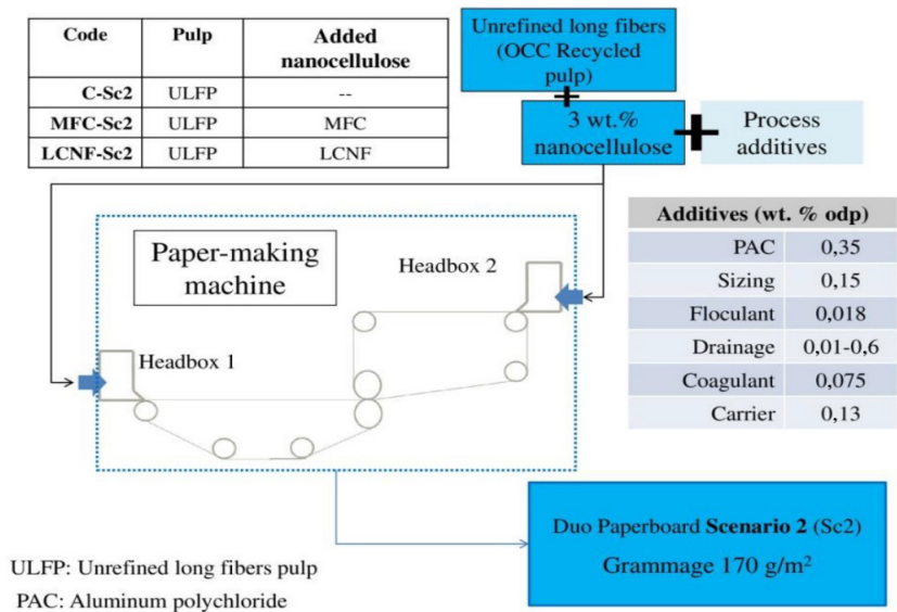
Figure 2: Scenario 2 defined for the production of 170 g/m² paperboard from ULFP and nanocellulose
