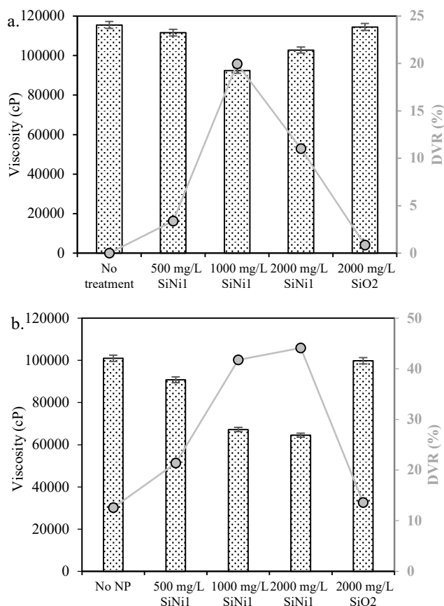
Figure 3. Effect of SiNiI nanoparticle dosage (0, 500, 1000, and 2000 mg/L) and SiO 2 support (2000 mg/L) on the HO viscosity reduction for a) no ultrasound treatment, b) after ultrasound exposure. Exposure time = 90 minutes; Temperature = 25 °C and 10 s -1 . Source: The authors.
