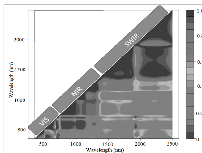
Figure 2. Pearson correlation between wavelengths.
