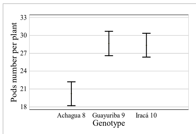
Figure 1. 95% Confidence intervals, Bonferroni comparator for each of the means
