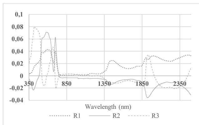
Figure 3. Weights of the values of the wavelengths in each factor.
