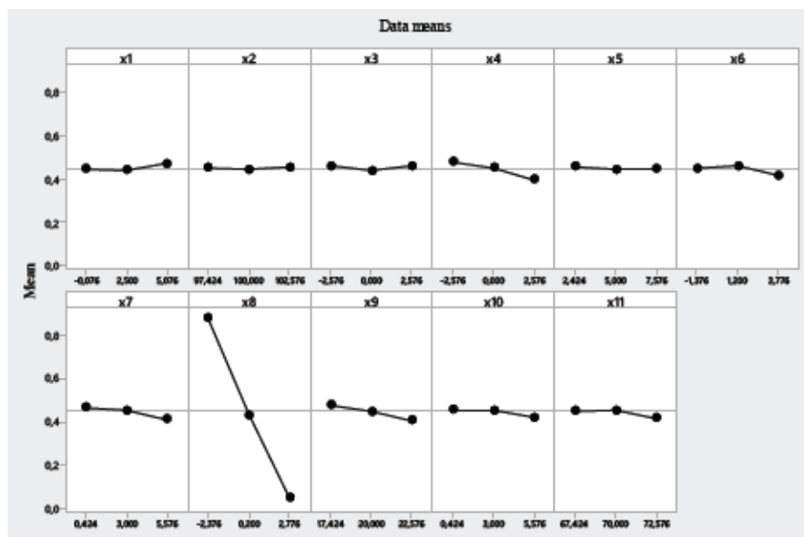
Figure 4 Main effects for five-hour IVR model Source: The Authors.
