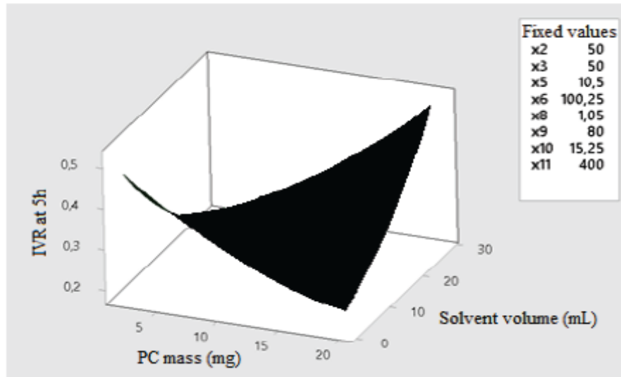
Figure 5 Effect of the relation between PC mass - solvent volume over the five-hour IVR Source: The Authors.
