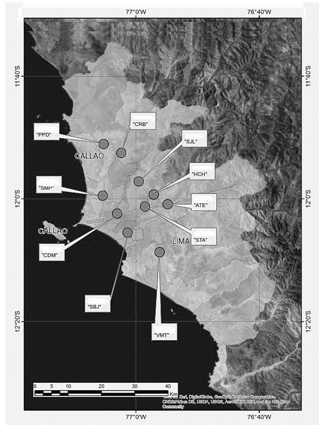
Figure 1. Air quality monitoring stations, Lima and Callao. Source: The authors
