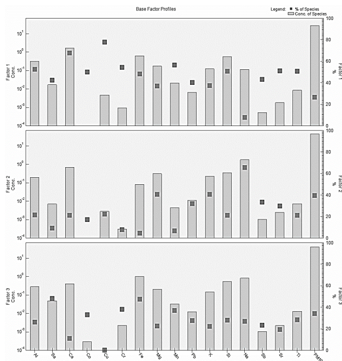
Figure 5. Source factors for PM 10 in the SJL district. Source: The Authors.
