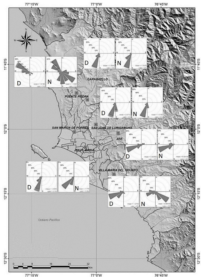
Figure 3. SENAMHI Monitoring Network, wind roses for April-May 2017. D, N= daytime and night. Source: The Authors.
