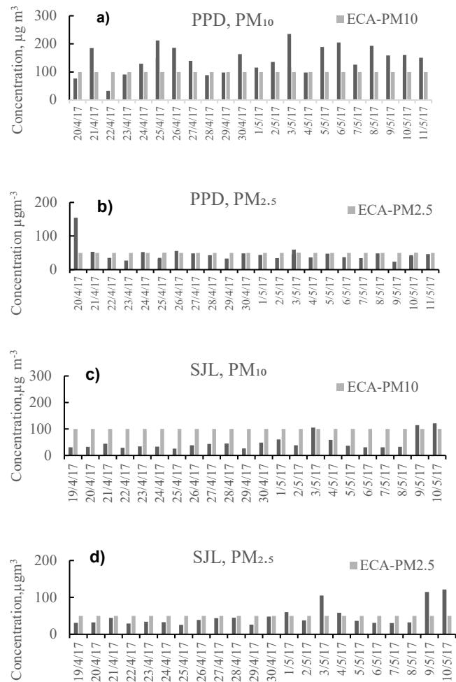
Figure 2. PM10 Concentrations in the PPD (a, b) and SJL (c, d) districts. Source: The Authors.
