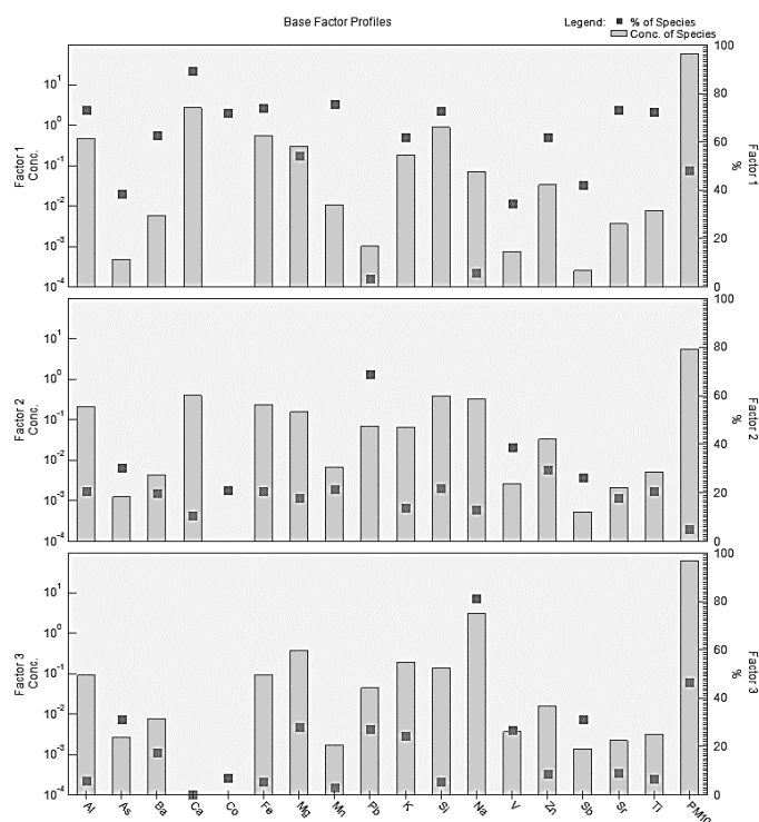
Figure 4. Source factors for PM 10 in the PPD district. Source: The Authors.
