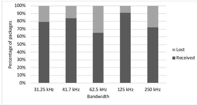
Figure 7. Probability of received and lost packages discriminated per bandwidth. Source: The authors.
