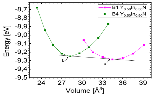
Figure 5. Energy vs. volume for the compound YInN
