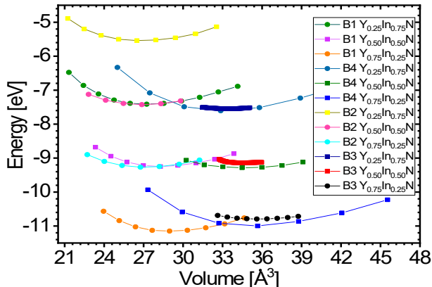
Figure 1. Energy vs. volume for the compound YInN
