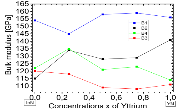
Figure 4. Bulk modulus vs. concentrations x of yttrium
