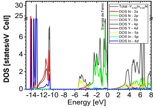
Figure 14. DOS partial and total for Y_{0.50}In_{0.50}N in the B4 after of the phase transition Y_{0.50}In_{0.50}N in the B1. Source: The Authors
