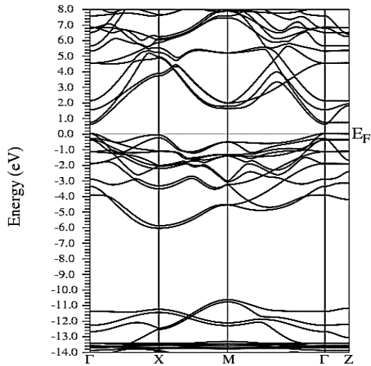
Figure 15. Electronic bands for Y_{0.50}In_{0.50}N in the B1 before of the phase transition to Y_{0.50}In_{0.50}N in the B4. Source: The Authors
