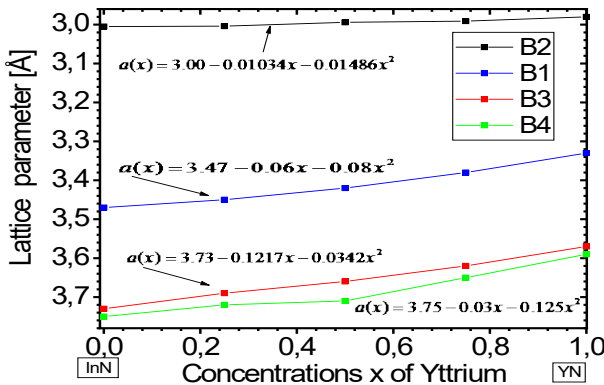
Figure 3. Lattice parameter vs. concentrations x of yttrium
