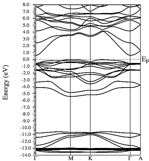
Figure 16. Electronic bands for Y_{0.50}In_{0.50}N in the B4 after of the phase transition Y_{0.50}In_{0.50}N in the B1. Source: The Authors
