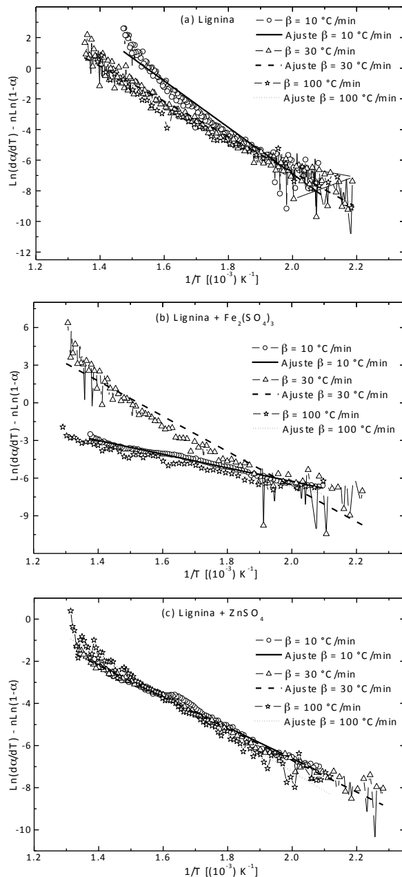
Figure 3. Fit to the n reaction order model for lignin with and without catalysts.
