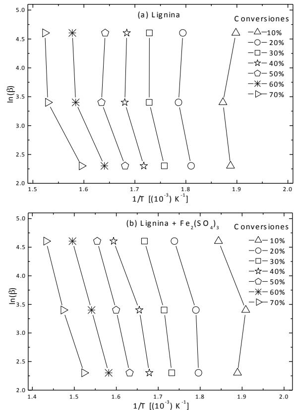
Figure 4. Isoconversional method for lignin with and without catalysts.
