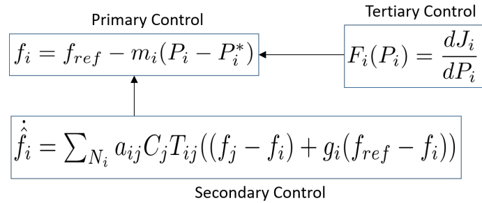
Figure 2. Hierarchical control layers
