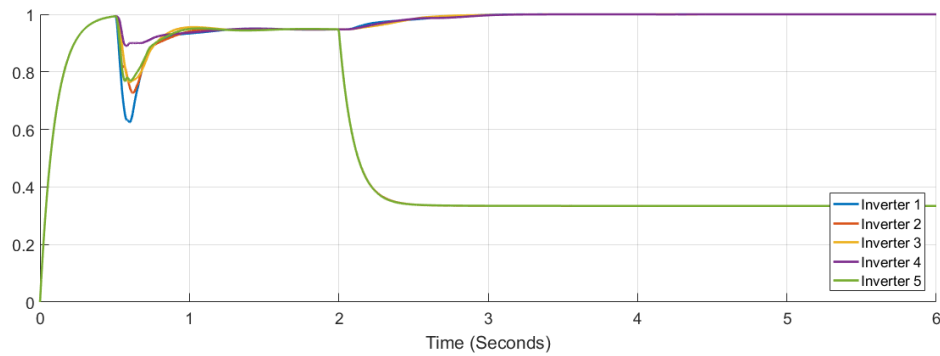
Figure 19. Confidence factor when inverter 1 is under attack
