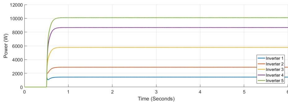
Figure 16. Output from the tertiary controller when is under attacks in case 3
