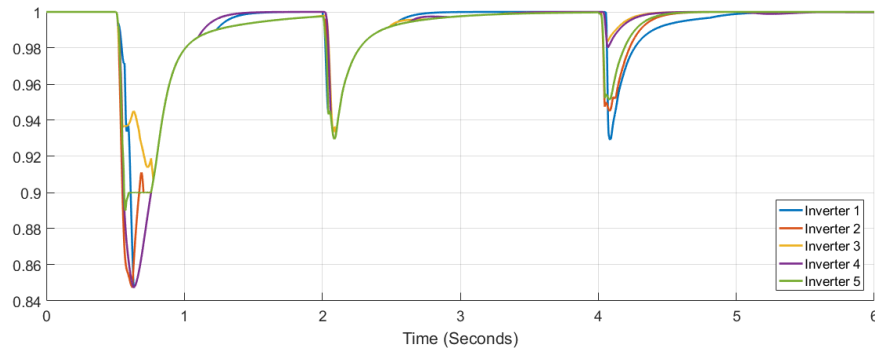
Figure 14. Trust factor when inverter 2 is under attack
