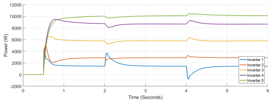
Figure 10. Active power for each inverter under attack in case 2
