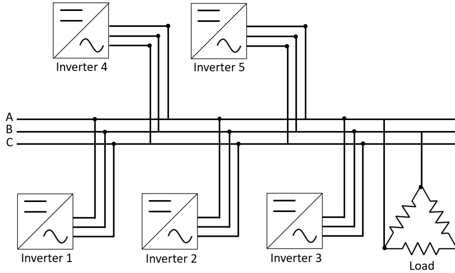
Figure 3. Microgrid Schematic
