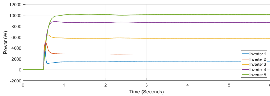
Figure 15. Active power for each inverter under attack in case 3
