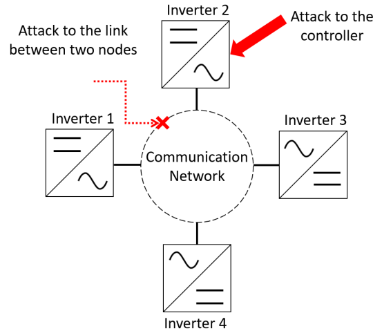
Figure 1. Types of attacks in a microgrid
