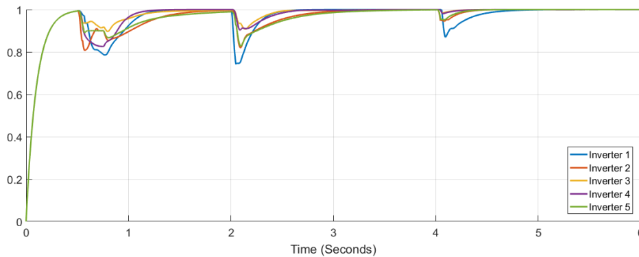
Figure 13. Confidence factor when inverter 1 is under attack
