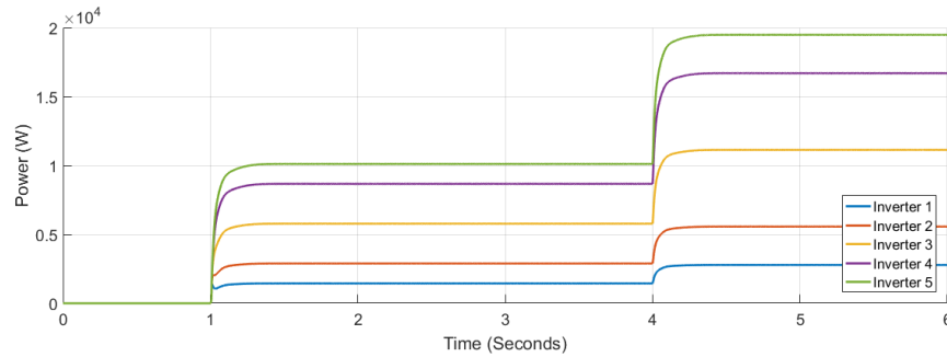
Figure 6. Output from tertiary controller
