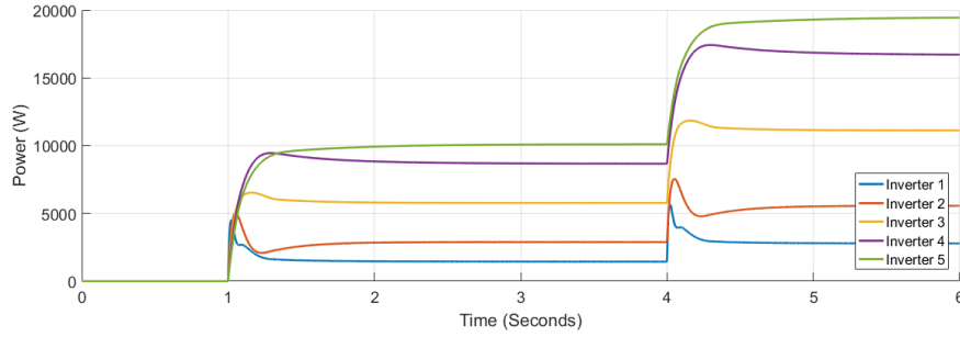
Figure 5. Active power for each inverter
