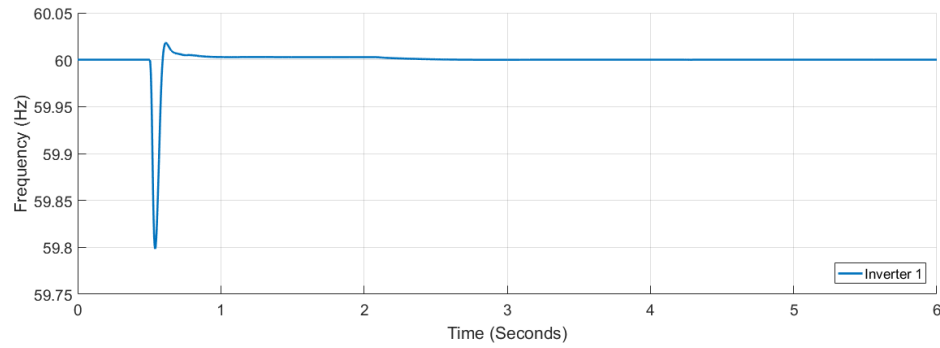
Figure 18. Frequency measured at inverter 1 under attack
