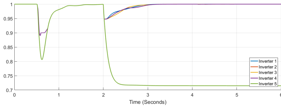
Figure 20. Trust factor when inverter 3 is under attack
