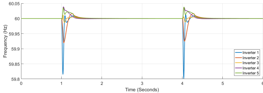
Figure 7. Frequency measured at each inverter
