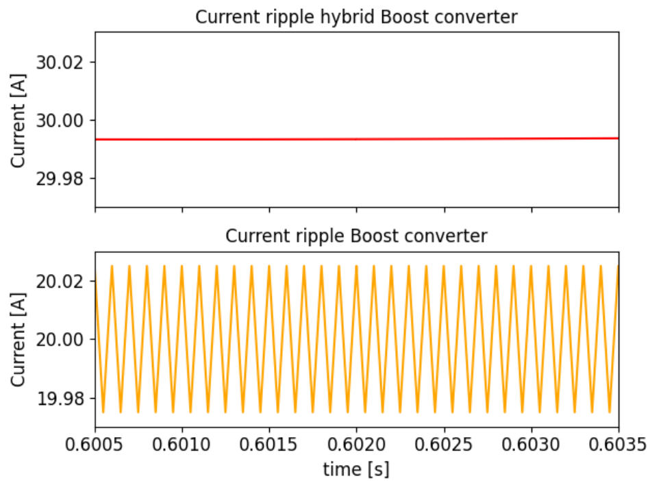
Figure 16. Current ripple
