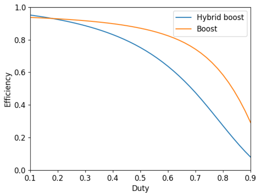
Figure 17. Efficiency
