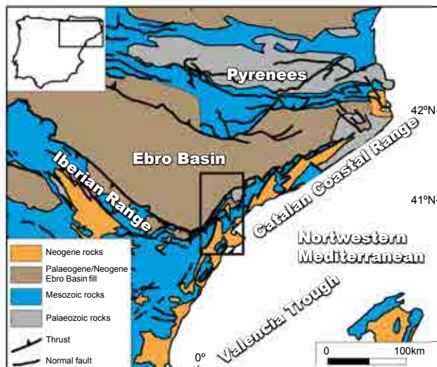
FIGURE 1. Location of the study area (black-framed inset) in the framework of the NE Iberian Peninsula, the Catalan Coastal Range (CCR) and the Catalan part of the NE Iberian continental Margin that makes up the NW margin of the Northwestern Mediterranean Basin.
