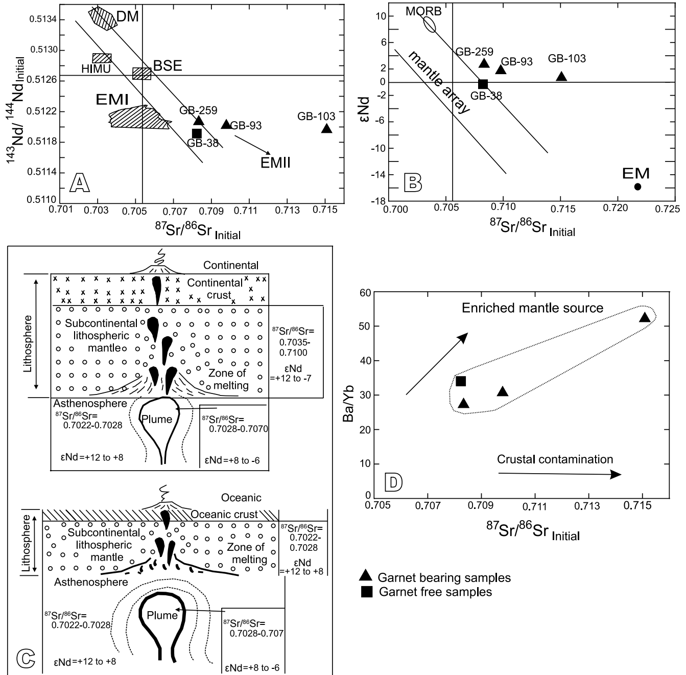
FIGURE 11. A) Initial ^{87}\text{Sr}/^{86}\text{Sr} vs. initial ^{143}\text{Nd}/^{144}\text{Nd} diagram. B) \epsilon\text{Nd} values vs. initial ^{87}\text{Sr}/^{86}\text{Sr} diagram. In A and B, the studied samples plot on the lower right quadrant. C) Comparison between Sr and Nd isotopic ratios in active continental rift basalts and oceanic island basalts (McDonough et al. , 1985). D) In the diagram of initial ^{87}\text{Sr}/^{86}\text{Sr} vs. Ba/Yb, the sources of Gol-e-Gohar metabasites show an enrichment trend. Abbreviations: DM: Depleted Mantle, EM: Enriched Mantle, HIMU: A source with a High ^{238}\text{U}/^{204}\text{Pb} , BSE: Bulk Silicate Earth according to Zindler and Hart (1986).
