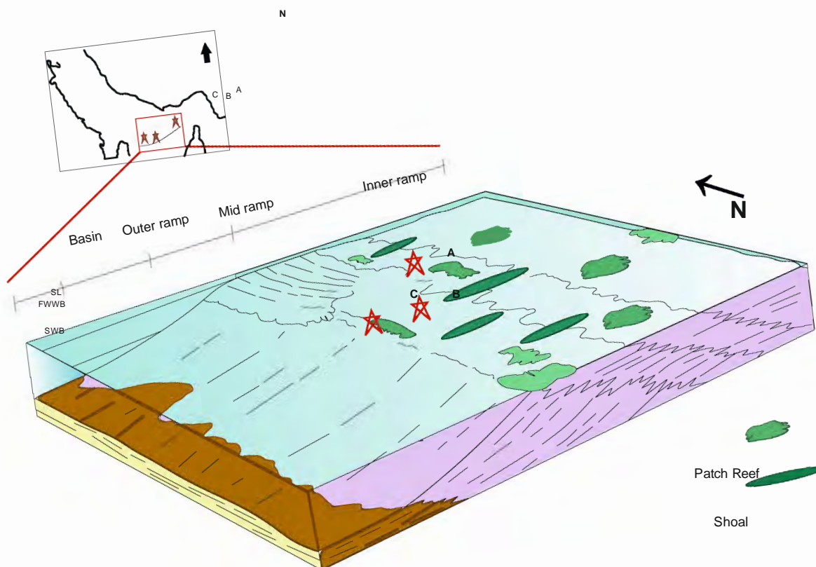
FIGURE 4. Approximate situation of the studied wells on a homoclinal ramp model of the Mishrif-Khatiya based on the frequency of identified carbonate facies.
