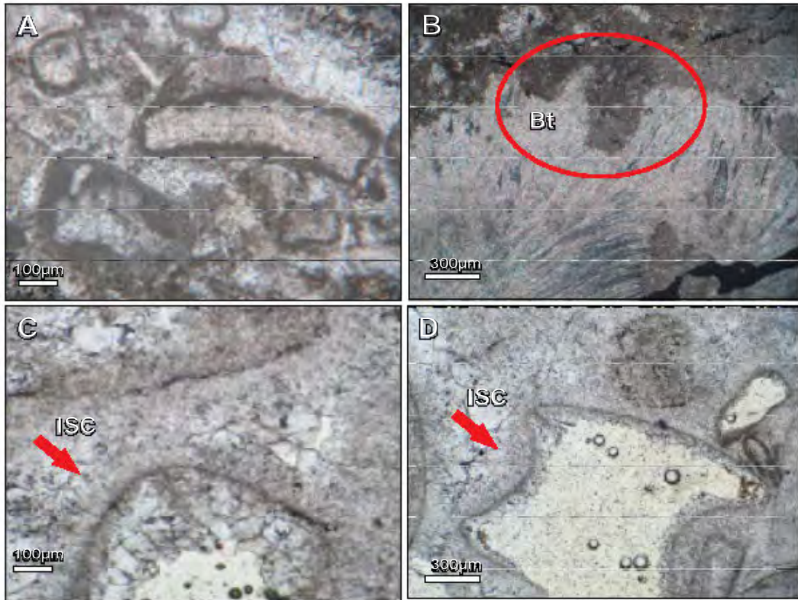
FIGURE V. Marine environment diagenetic processes. A) Micritization. B) Bioturbation (boring). C- D) Thin isopachous microcrystalline calcite cement. (All in PPL, X5).
