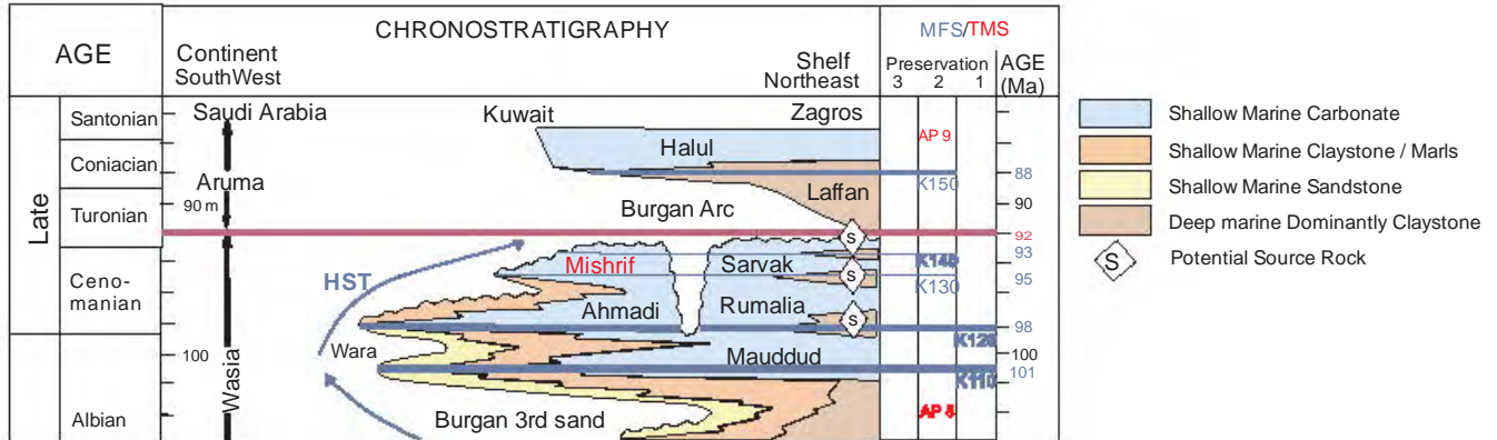
FIGURE I. Chronostratigraphic chart of the mid- and late-Cretaceous in the Arabian Plate (modified after Sharland et al. , 2001).
