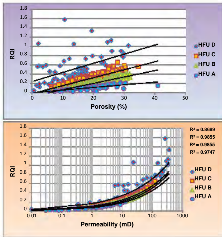
FIGURE VIII. Relationship between Reservoir Quality Index (RQI) with porosity (A) and permeability (B) for different hydraulic flow units in the reservoir.
