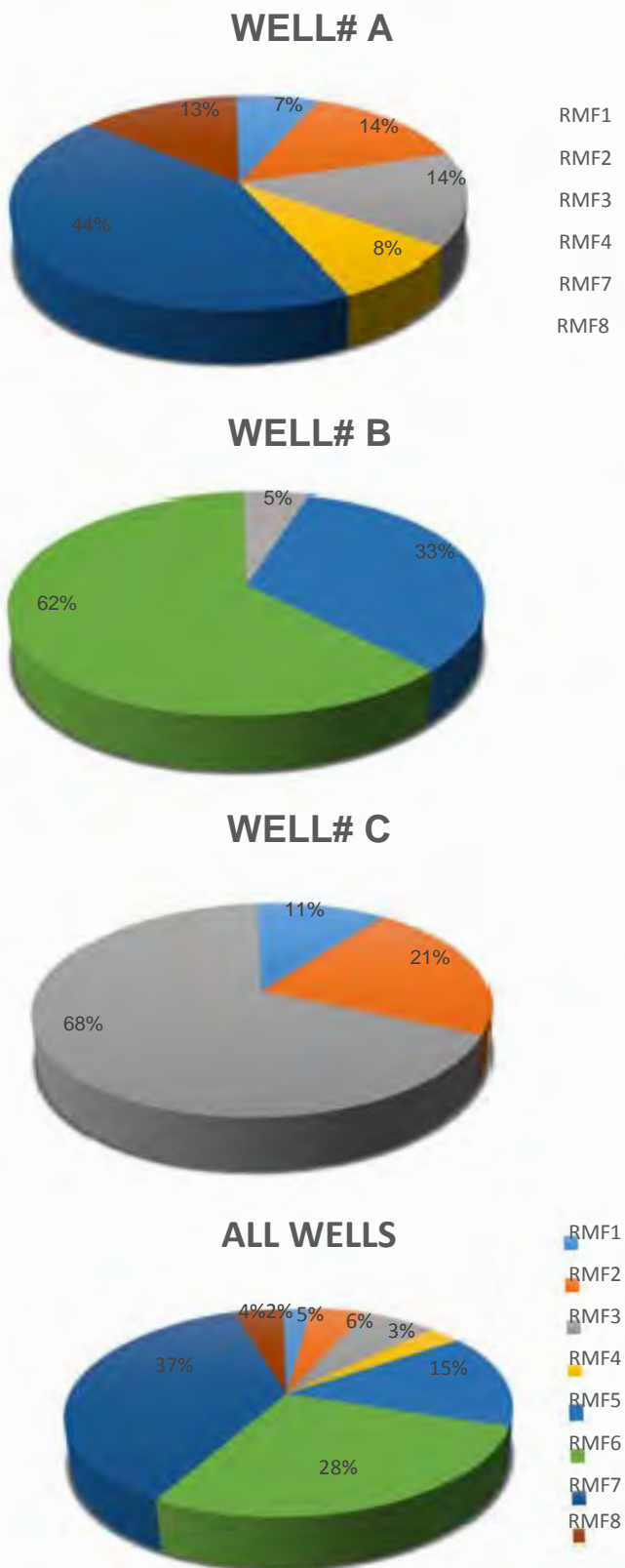
FIGURE III. Pie diagrams showing the frequency (percent) of different microfacies (RMFs) identified in three studied fields.
