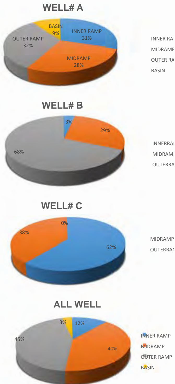
FIGURE IV. Pie diagrams showing the frequency (percent) of different facies belts (FBs) identified in three studied fields.
