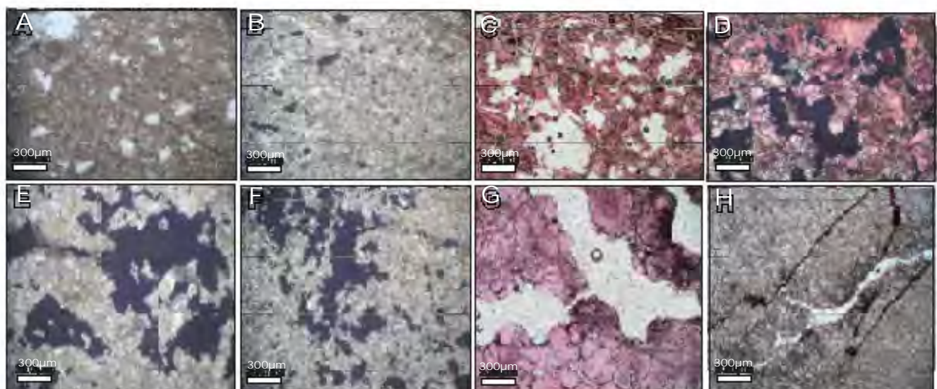
FIGURE X. A-B) HFUA, with high-porosity and low-permeability and non-attached vugs and moldic pores resulted from meteoric dissolution. C-D) HFUB, with intermediate poroperm and most of the pore spaces are touching vugs. E-F) HFUC (are similar to HFUB). G-H) HFUD, with high-quality especially with high-permeability and low-porosity related touch and non-touching micro vugs to because of open fracture and burial dissolution. (A, C, G and H are in PPL and X5. B, D, E and F are Double (or crossed) Polarized Light (XPL) and X5).
