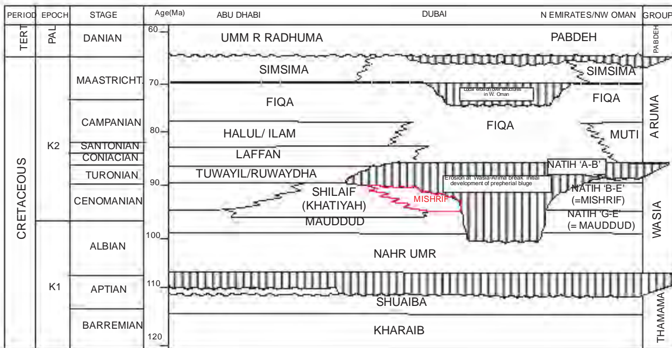
FIGURE 1. Chronostratigraphic chart of the mid-Cretaceous in the South Persian Gulf and Oman (Haq et al. , 1988).
