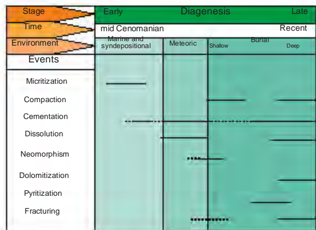
FIGURE 6. Paragenetic sequence of diagenetic processes illustrated for the Mishrif Fm. in the studied fields.
