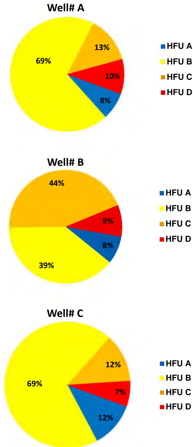
FIGURE XI. Pie diagram showing the frequency of the identified flow units in the studied wells (A, B and C).
