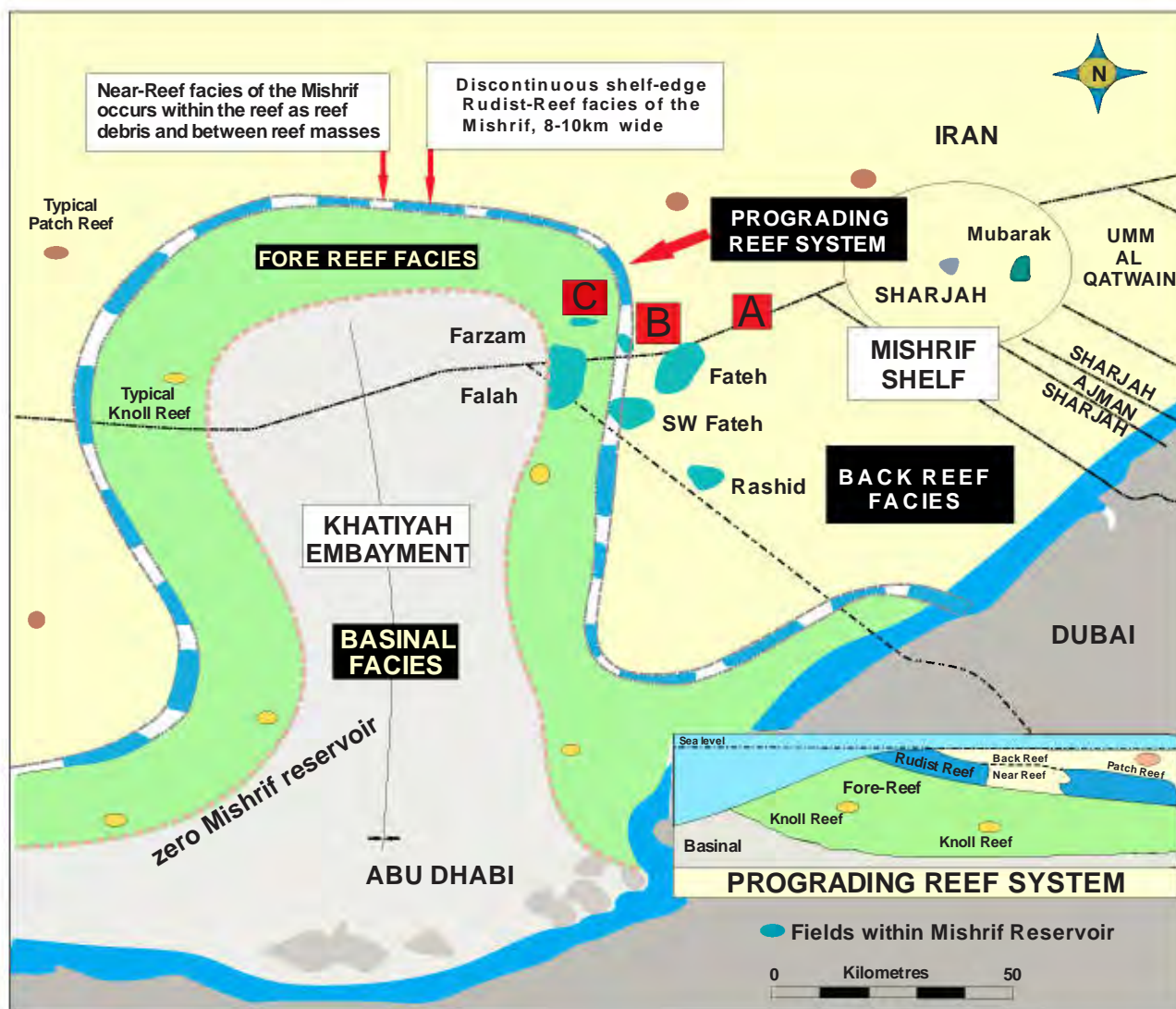
FIGURE 5. A schematic map illustrating development of the Khatiya Basin with marginal reefs (Mishrif) in the East of Persian Gulf, and the location of the studied fields (A, B and C) in this basin (Rezaee, 2002).
