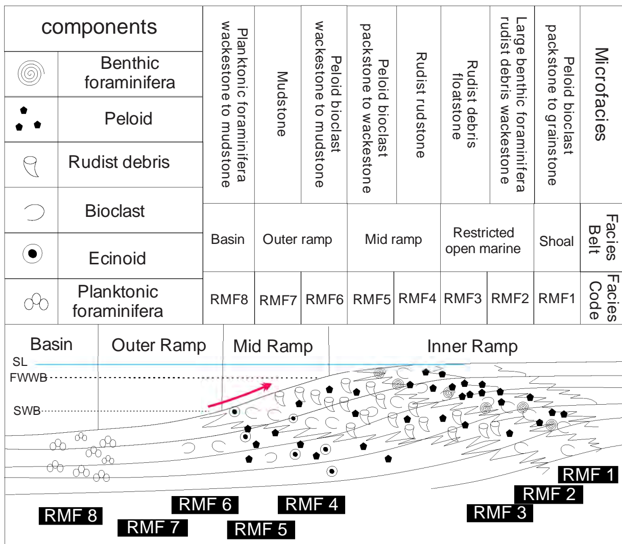
FIGURE 3. Depositional model (homoclinal ramp) for the Mishrif Fm. in the Sirri Oil field showing the distribution of microfacies and facies belts in different parts of the model. The arrow on this model indicates the shallowing upward trend of facies.
