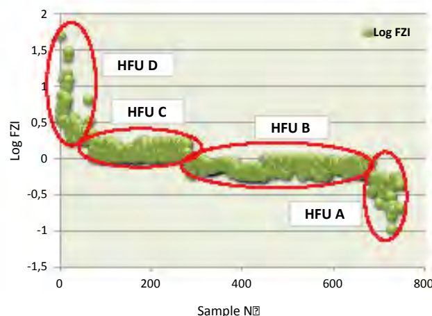
FIGURE 8. Log Flow Zone Indicator (FZI) versus sample numbers for determination of hydraulic flow units in the reservoir.
