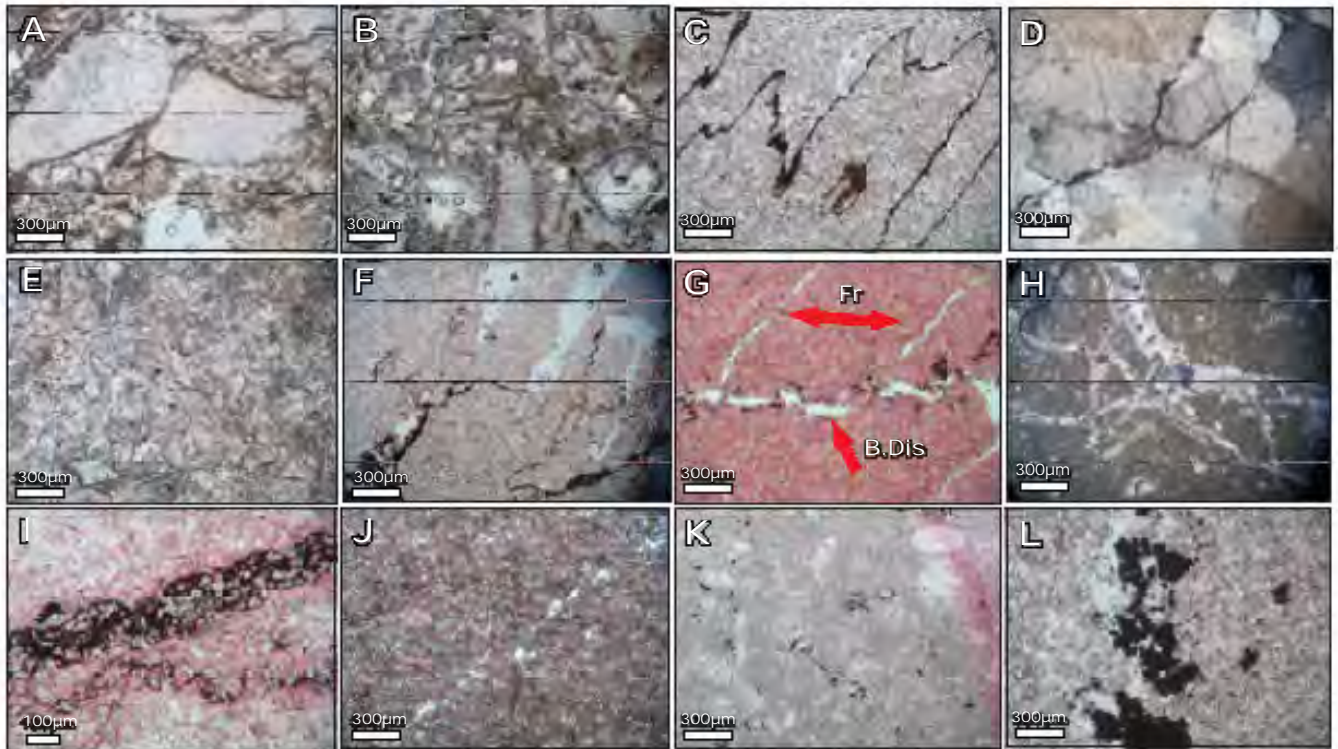
FIGURE VII. Burial environment diagenetic processes. A-B) Physical compaction. C) High-amplitude stylolite. D-E) Burial cementation with coarse crystal and sharp cleavages. F-G) Burial dissolution, occurrence of solution on stylolite. G-H) Fracturing (open and filled). I) Dolomitization related to solution seams with fine- to medium-size and euhedral to subhedral crystals. J) Sparse dolomitization with very fine- to medium-size and euhedral to subhedral crystals in micrite of mud-dominated facies. K-L) Secondary pyritization. (All in PPL and X5).
