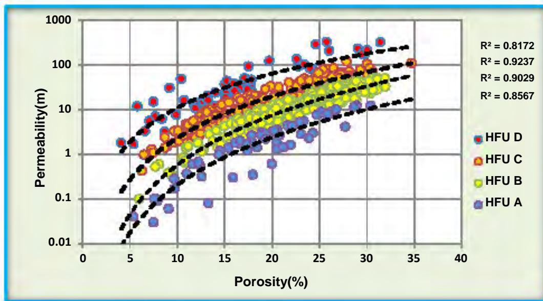
FIGURE IX. Distribution of different hydraulic flow units on porosity and permeability plot for the Mishrif reservoir.
