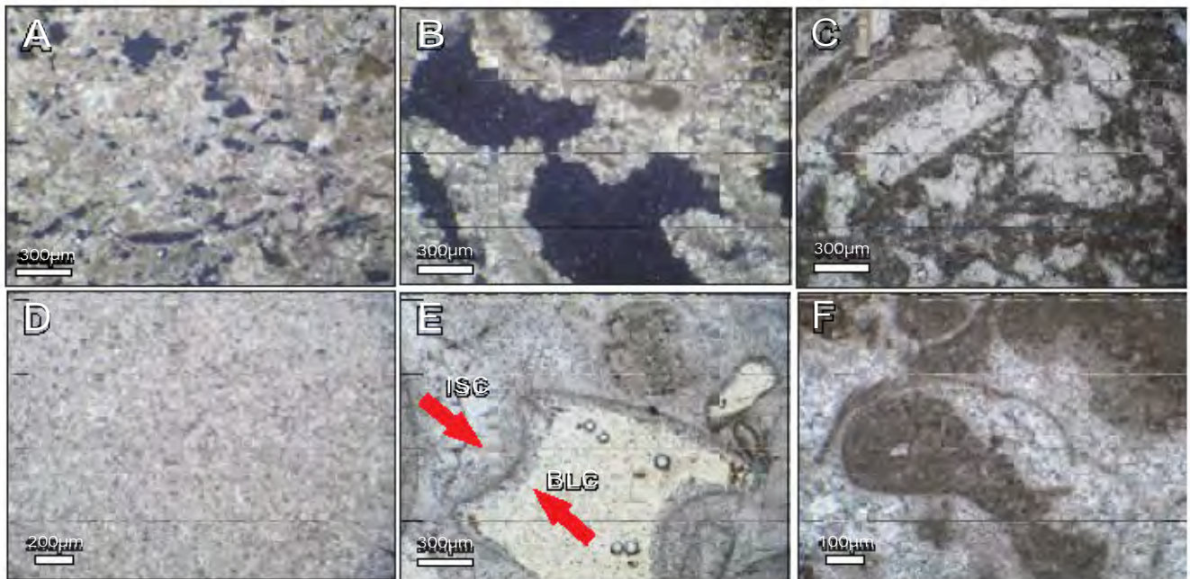
FIGURE VI. Meteoric environment diagenetic processes. A-B) Meteoric dissolution (in xpl and X5). C-D) Neomorphism (in PPL and X5). E) Meteoric cementation (in PPL and X5). F) Geoptal fabric (in PPL and X5).
