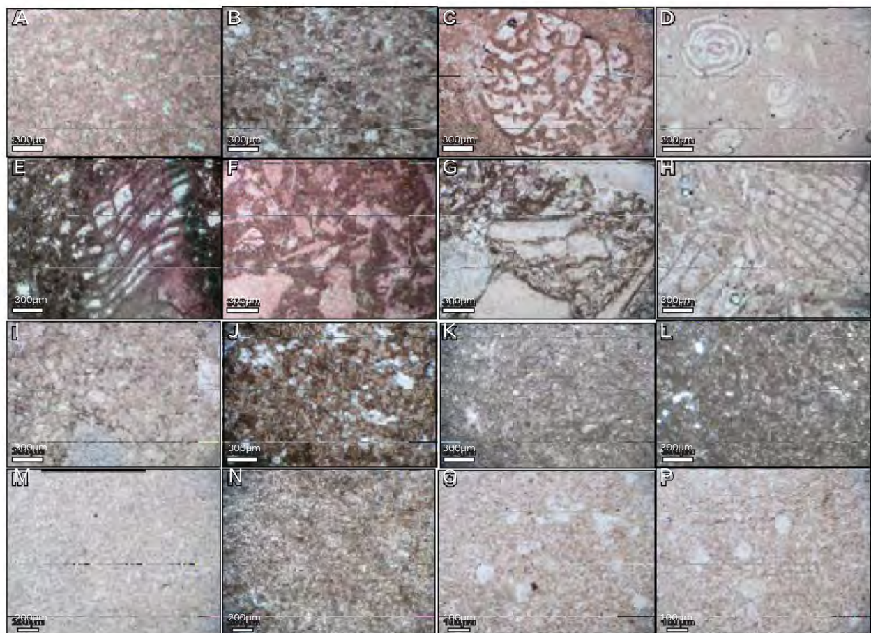
FIGURE II. Identified microfacies of the Mishrif Fm. in the studied fields. A-B) RMF1, peloidal/bioclastic packstone to grainstone. C-D) RMF, large benthic foraminifera wackestone with rudist debris. E-F) RMF3, rudist debris floatstone. G-H) RMF4, rudist rudstone. I-J) RMF5, peloid bioclast packstone/wackestone. K-L) RMF6, peloid bioclast wackestone/mudstone. M-N) RMF7, mudstone. O-P) RMF8, planktonic foraminifera wackestone/mudstone. All figures are in Plane Polarized Light (PPL) and X5.
