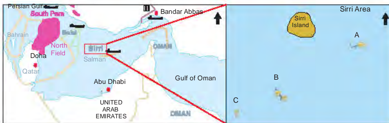
FIGURE 2. Location map of the studied fields (A, B and C) in the Persian Gulf.
