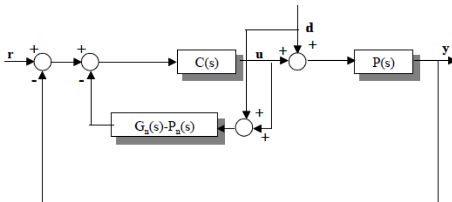
FIGURA 2 Forma simple del feedforward SP
