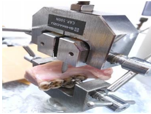
Figure 1. Mounting in the texture analyzer to measure shear force in a pig mandible (lateral view).
