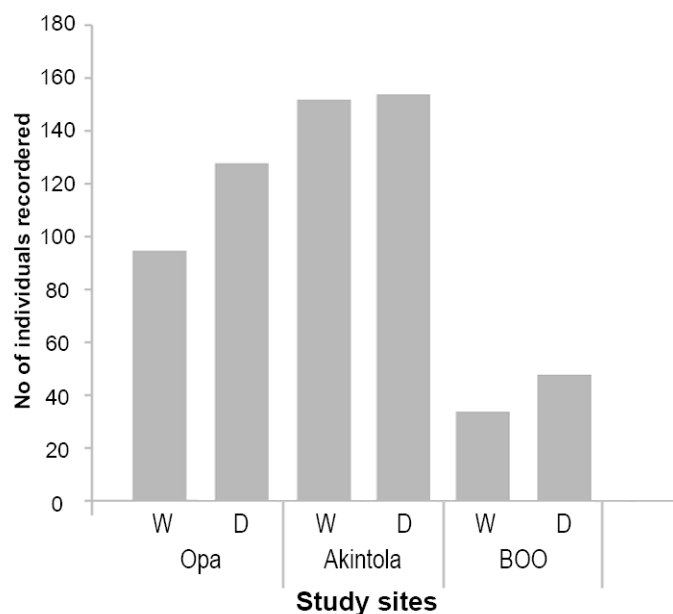
Fig. 1. Seasonal abundance of mosquitoes in Obafemi Awolowo University, Ile - Ife (W- WET SEASON; D - DRY SEASON).
