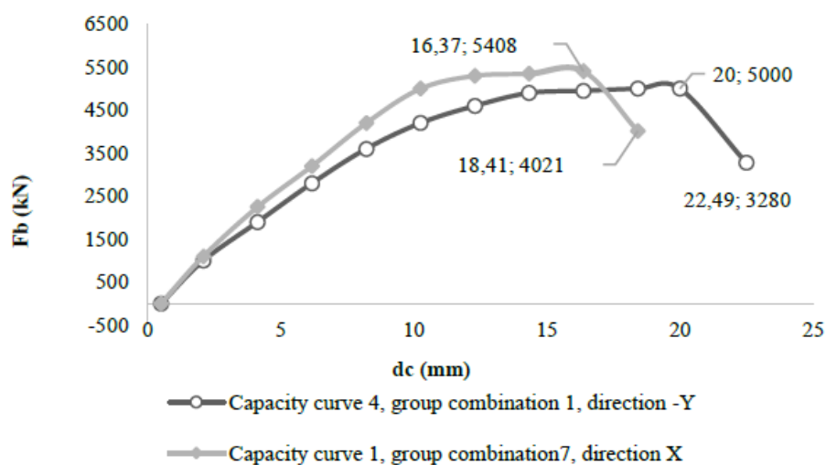
FIGURE 6 . Sismicad12 capacity curve.
