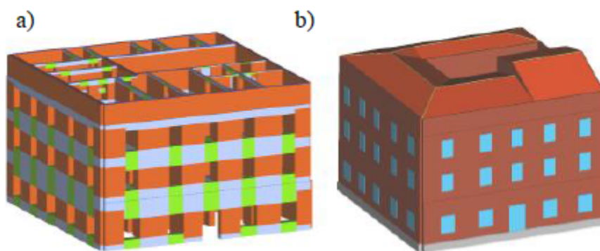
FIGURE 4 . 3Muri simulation overview: a) FEM model; b) 3D model.
