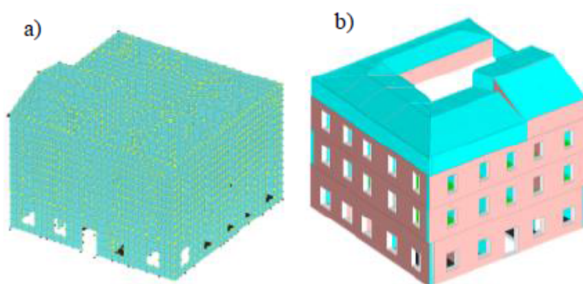
FIGURE 2 . Sismicad12 simulation overview: a) FEM model; b) 3D model. Own elaboration.
