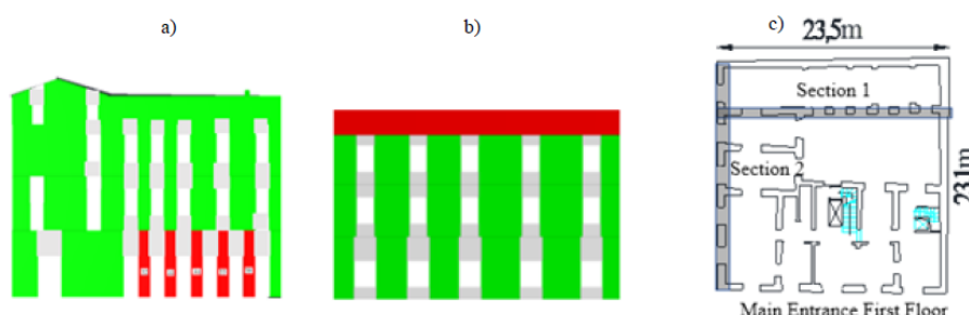
FIGURE 3 . Results of the review of the most critical sections: a) Section 1; b) Section 2; c) First floor.
