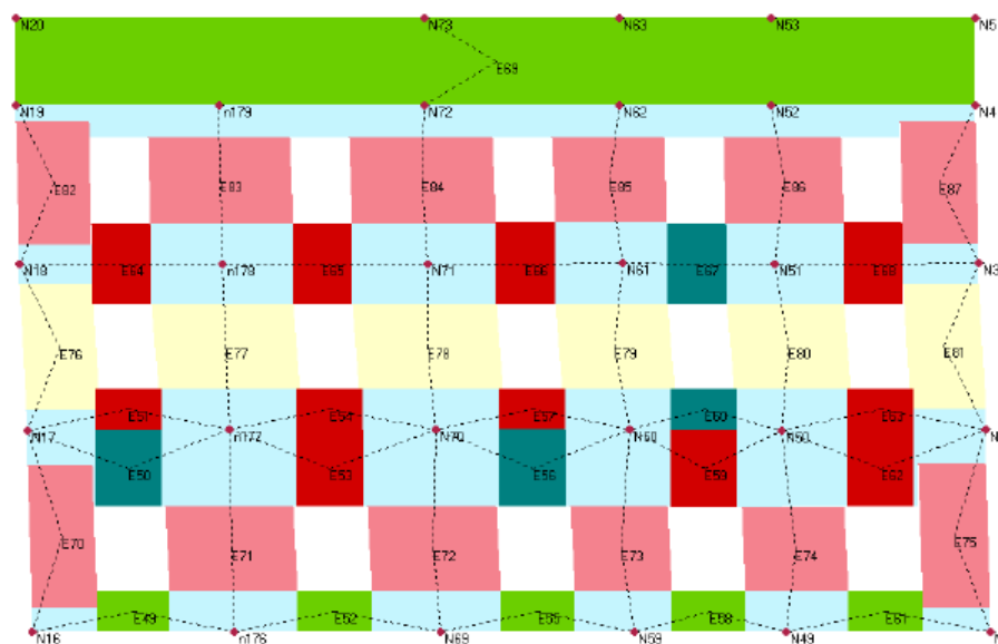
FIGURE 10. Decay of the structure capacity of 3Muri in a representative section.
