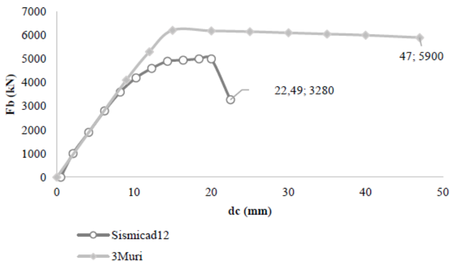
FIGURE 8 . Comparison of capacity curves similarly loaded.
