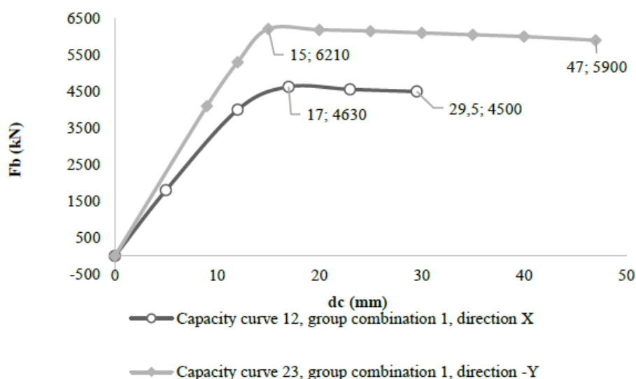
FIGURE 7 . 3Muri capacity curve
