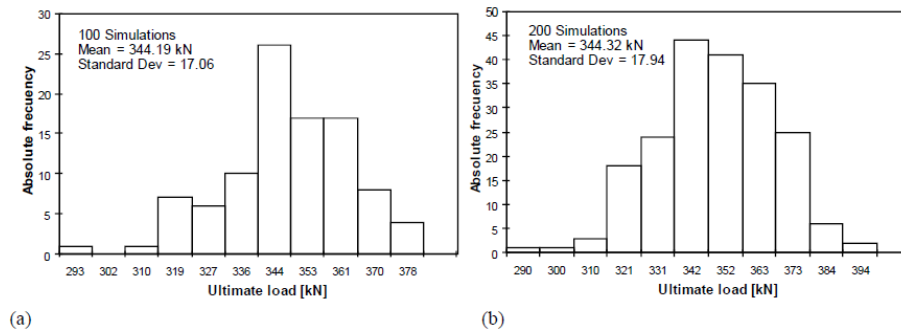
Figure 5. Histogram for the ultimate load. L_e = 3m . (a) 100 simulations, (b) 200 simulations.
