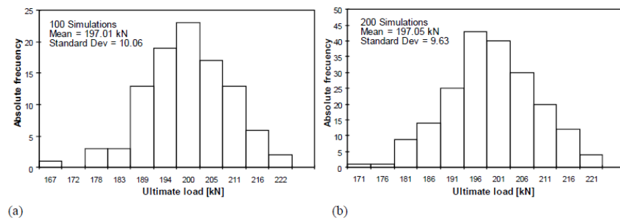
Figure 6. Histogram for the ultimate load. L_e = 4m . (a) 100 simulations, (b) 200 simulations.
