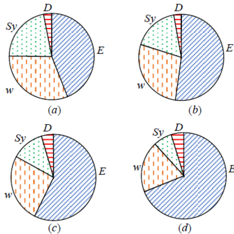
Figure 7. Sensitivity of the ultimate load for the column. (a) L_e = 2m , (b) L_e = 2.5m , (c) L_e = 3m , (d) L_e = 4m .
