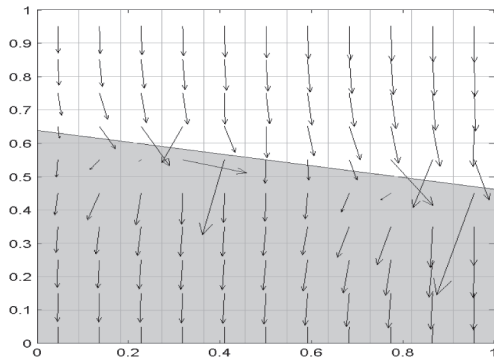
(a) FEM
