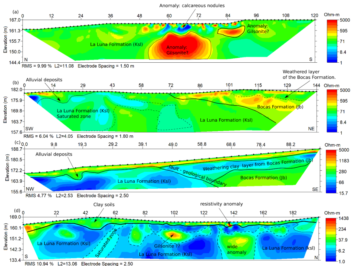
Figure 5. Interpretation of the electrical tomography data identifying main high resistivity anomalies corresponding to gilsonite occurrence. (a) ERT-1, (b) ERT-2, (c) ERT-3 and (d) ERT-4. Low resistivity anomalies are mainly associated with water saturated zones and characterize the moisture content of Ksl and Jb, and the highest resistivity anomaly is related to gilsonite bodies. Source: The authors. Image modified with the authorization of the company LAVGR SAS.
