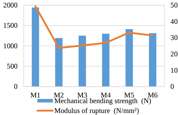
Figure 4. Mechanical resistance
