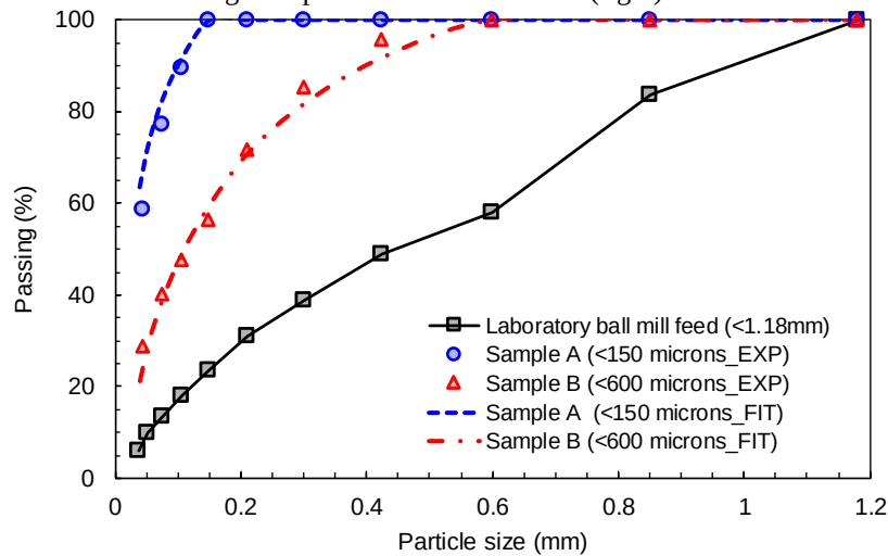
Figure 7. Laboratory ball mill feed <1.18mm and grinding product samples A (< 150 μm) and B(< 600 μm) experimental and simulated.
