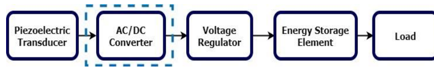
Figure 1. Schematic view of the main components of a typical piezoelectric energy harvester with AC/DC converter and storage system [9].
