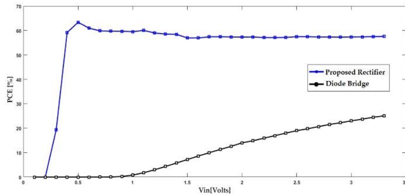
Figure 10. Results of the PCE of proposed CMOS rectifier and a D1N4148 diode bridge circuit. For both rectifier circuits, a frequency of 200Hz and a load resistance of 45 k \Omega were considered.
