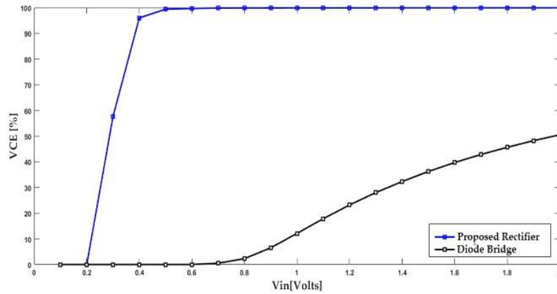
Figure 9. Results of the VCE of proposed CMOS rectifier and a D1N4148 diode bridge circuit. For both rectifier circuits, a frequency of 200Hz and a load resistance of 45 K \Omega were considered.
