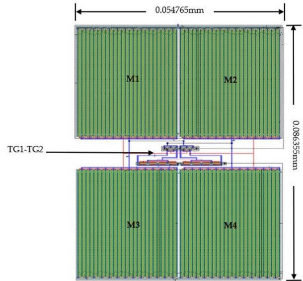
Figure 5. Layout of the proposed CMOS rectifier with transmission gates.
