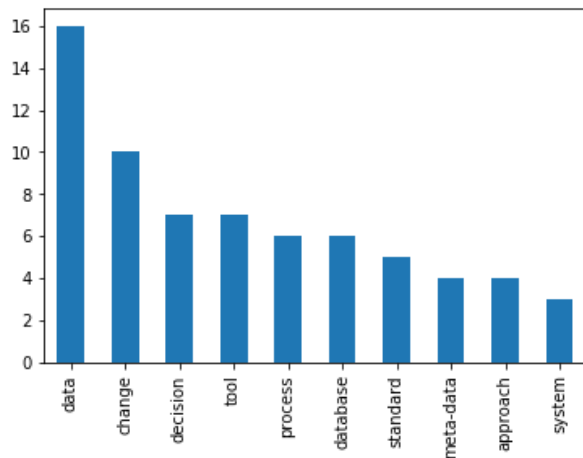
Figure 7. 10 Most common nouns extracted from the target-corpus. Source: authors.
