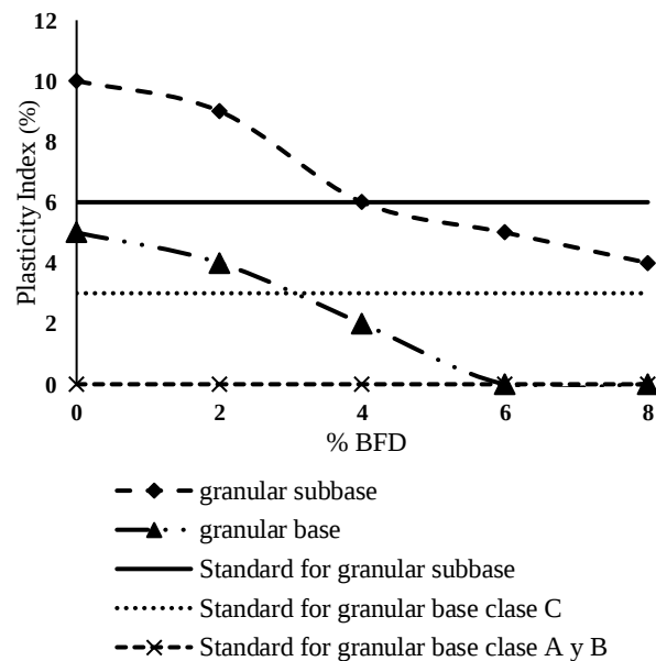
Figure 4. Behavior of the plasticity index.
