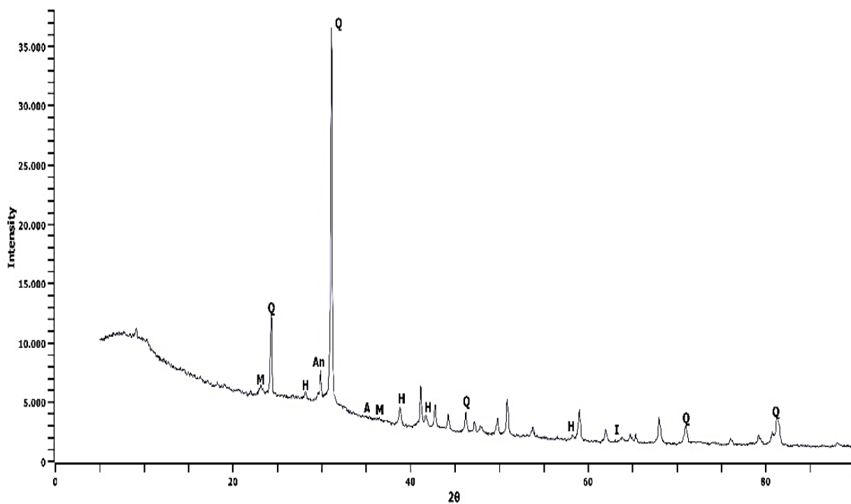
Figure 3. Diffractogram of CBA3. Q-Quartz; M-Muscovite; H-Hematite; An-Anatase; A-Andradite; I-Ilmenite. Source: own elaboration.
