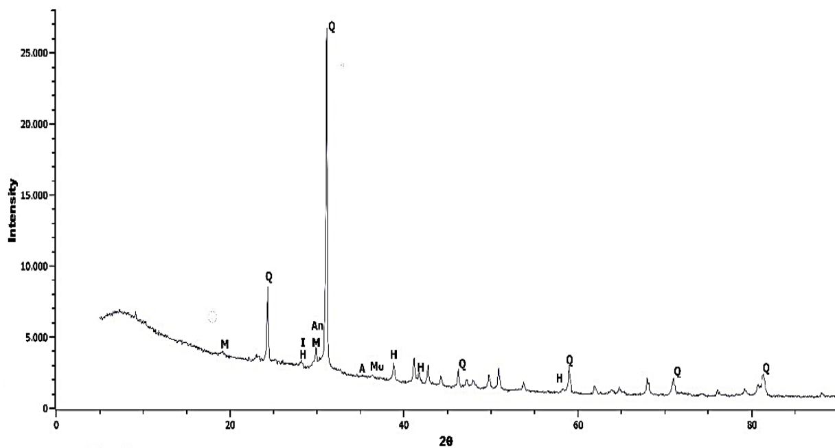
Figure 2. Diffractogram of CBA2. Q-Quartz; Mu-Muscovite; H-Hematite; An-Anatase; A-Andradite; I-Ilmenite; M-Mullite. Source: own elaboration.
