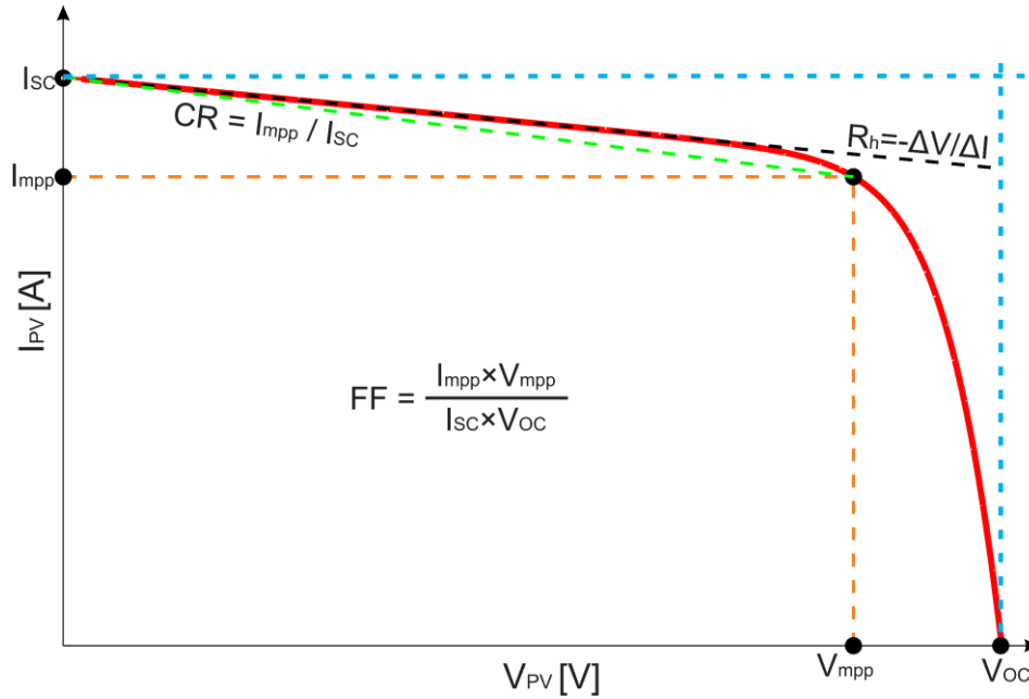
Figure 2. Graphical representations in the I-V curve associated with PID in PV panels: current ratio ( CR ), fill factor ( FF ), parallel resistance ( R_h ), and the points used to calculate them.
