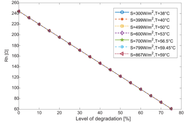
Figure 7. Estimation of R_h for reductions in R_h from 5% to 75 % at different irradiances and temperatures.
