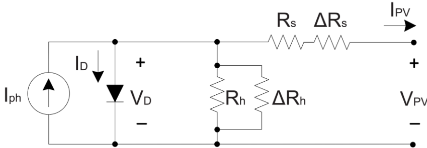
Figure 3. Single-diode model with degradation represented by additional series and parallel resistances, \Delta R_s and \Delta R_h , respectively [32].
