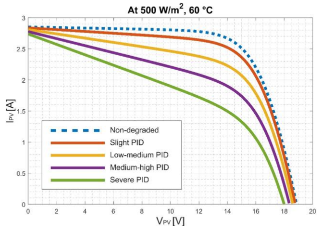
Figure 1. Light I-V curve of a PID-free PV panel (dash-dot blue line) and I-V curves of a PID-affected PV panel at different degradation levels.
