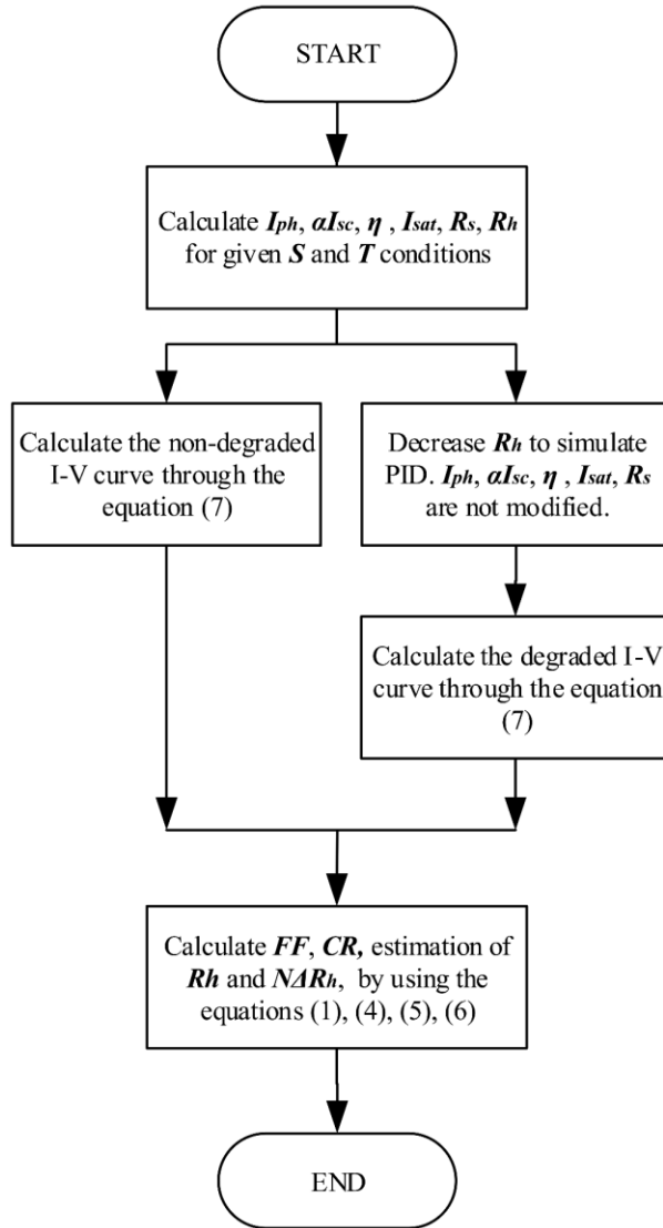
Figure 5. Flowchart of the PID simulation on a PV panel for given irradiance ( S ) and temperature ( T ) conditions.
