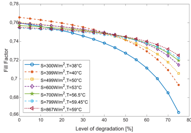
Figure 6. Fill Factor ( FF ) for reductions in R_h from 5% to 75 % at different irradiances and temperatures.
