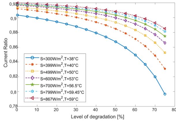
Figure 8. Current ratio ( CR ) for reductions in R_h from 5% to 75 % at different irradiances and temperatures.
