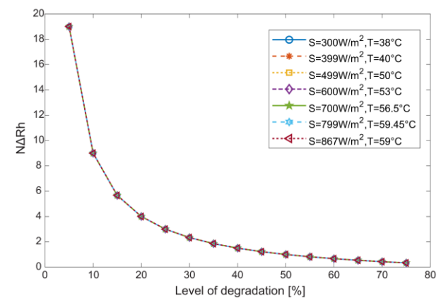
Figure 9. Normalized change of R_h ( N\Delta R_h ) for reductions in R_h from 5 % to 75 % at different irradiances and temperatures.
