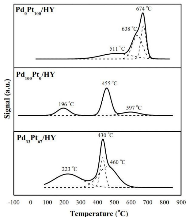
Figure 1. Hydrogen temperature-programmed reduction (H 2 -TPR) on Pd-Pt/HY catalysts.
