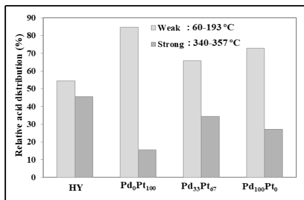
Figure 3. Relative Acid distribution (%) by NH 3 -TPD on Pd-Pt/HY catalysts.
