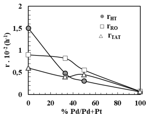
Figure 5. Rates of hydrogenation of toluene ( r_{HT} ), ringopening of methylcyclohexane ( r_{RO} ), and transalkylation of toluene ( r_{TAT} ) at 250 °C versus relative atomic Pd %.
