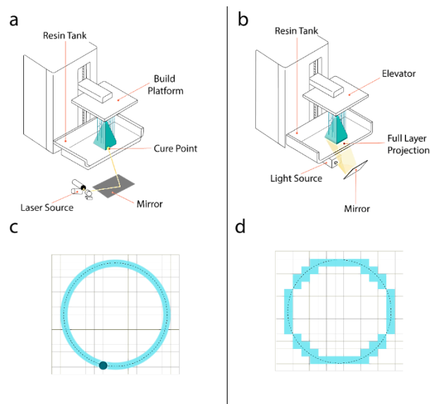
Figure 1. SLA vs DLP technologies. a) SLA apparatus set up. b) DLP apparatus set up. c) Laser beam sized resolution from SLA, in which a single point gets cured at a time without a pixelated effect. d) Display pixelated resolution from DLP, in which a complete projected geometry (layer) gets cured. Source: Author.
