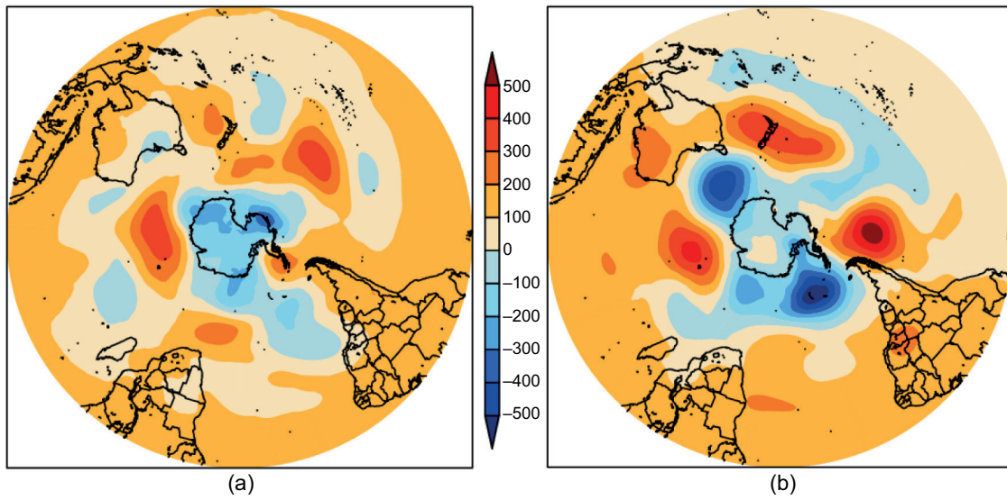
Fig. 2. Geopotential height anomalies at 700 hPa (mgp): (a) 2020 austral summer, and (b) 2019 austral summer. Data source: ERA5.
