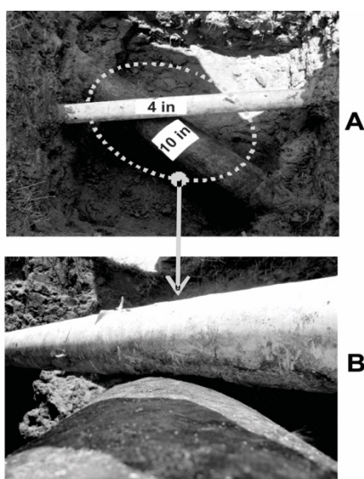
Figure 10. Excavation at X = 682 m of 4 in OD gas pipeline. A) Plan view of the excavation with pipelines crossing. B) Zoomed view of the contact between pipes that causes damage in the coating.
