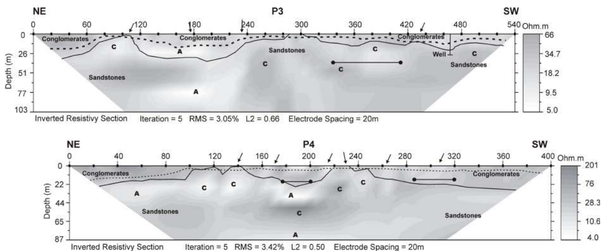
Figure 11. ERT of Sector 1 (P3 and P4). The profiles are located graphically according to their position in the field (see Figure 5). Continuous curved lines indicate boundaries between rocks and discontinuous curved lines indicate water table. The section of P3 from 0 to 280 m and the section of P4 from 0 to 230 m are located next to the bridge. Vertical line indicate well.
