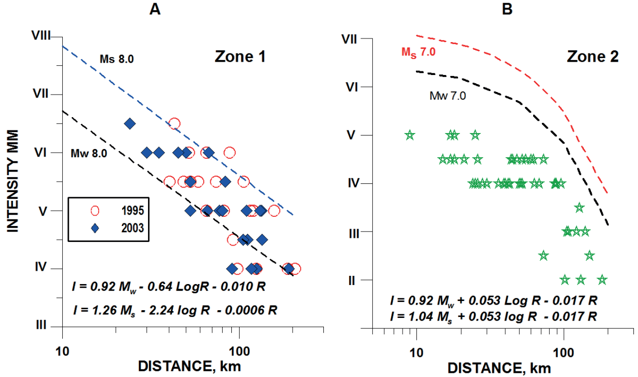
Figure 7. Attenuation of earthquake intensity with distance for events of Zone 1 (A) and Zone 2 (B). In A, the data are shown for large earthquakes of 1995 (No 7) and 2003 (No 8). The curves, calculated with equations, given in A, for earthquakes with magnitudes M_s 8.0 and M_w 8.0 , are shown. In B, the data are shown for the M_w 5.3 earthquake of 6 March 2000. The curves, calculated with equations, given in B, for earthquakes with magnitudes M_s 7.0 and M_w 7.0 , are shown.
