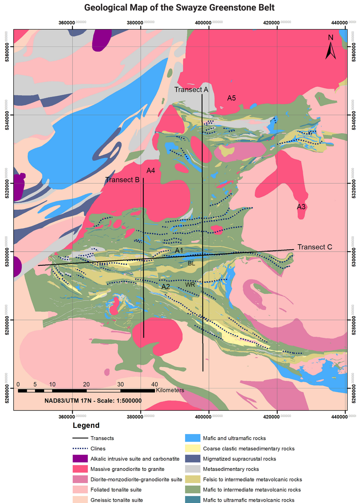
Figure 2. Geological map of the Swayze greenstone belt. Coordinate System NAD-83/ UTM Zone 17 N. The black solid lines indicate the traces of the profiles (transects) along which 2.75D forward modelling was conducted. BL and WR correspond to the Brett Lake and the Woman River folds, which are discussed in the text. In dark blue dashed lines are shown the axes of the different folds in the Swayze area. A1 to A5 indicate the different areas discussed in the Qualitative Analysis section. The digital geological dataset was downloaded in ArcGIS format from the website of the Ministry of Northern Development and Mines of Ontario: ( http://www.geologyontario.mndm.gov.on.ca/mndmaccess/mndm_dir.asp?type=pub&id=MRD126-REV1 ).
