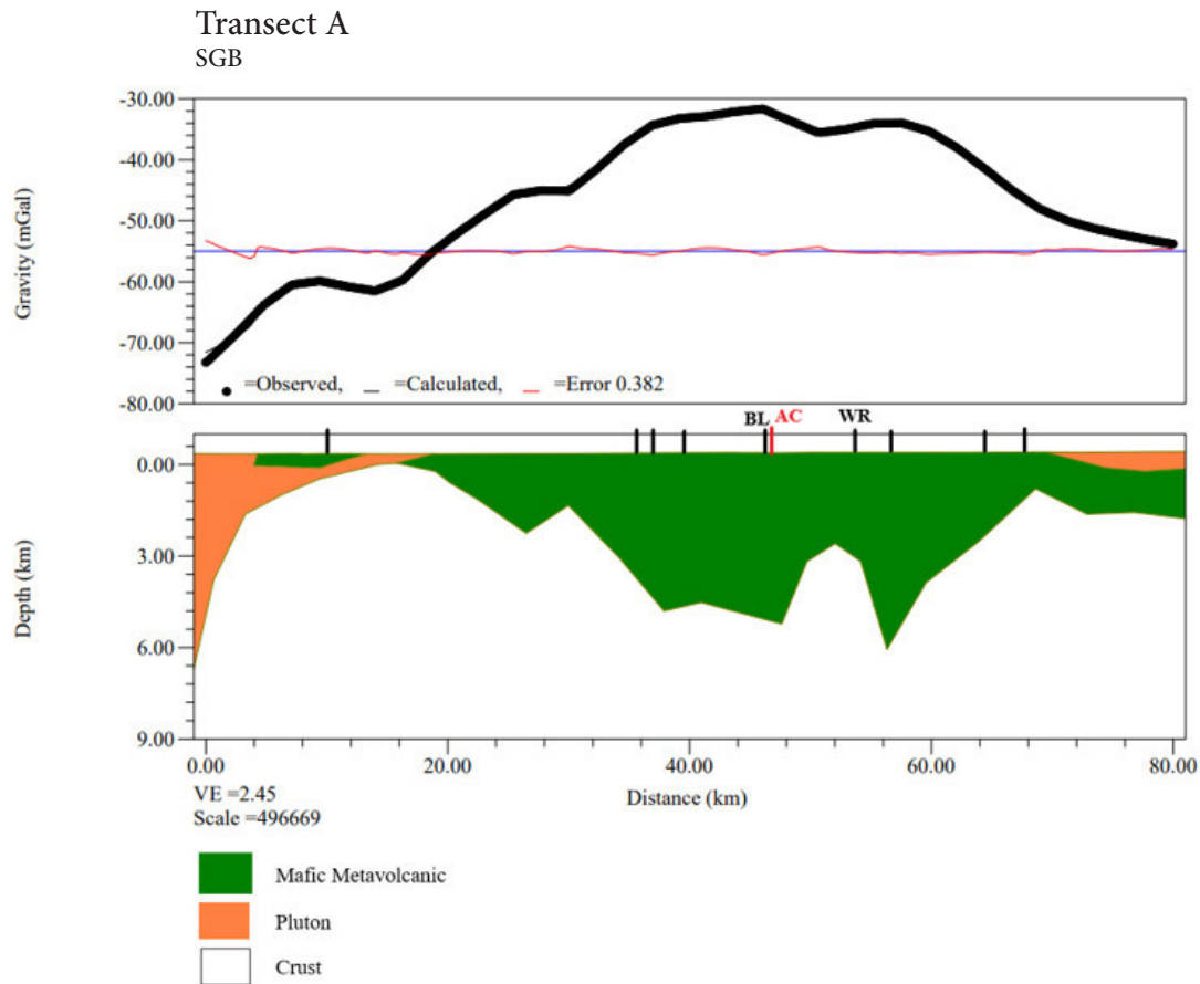
Figure 4. Gravity model along Transect A: Mafic Metavolcanic, \rho=2.89 \text{ g/cm}^3 ; Pluton, \rho=2.66 \text{ g/cm}^3 ; Crust, \rho=2.72 \text{ g/cm}^3 . The black vertical lines shown at the top of the model panel indicate the locations of the different fold axes crossed by the transect. The red vertical line represents the crossing location between Transect A and Transect C. WR-Woman River Anticline, BL-Brett Lake Syncline, AC-Crossing between Transect A and Transect C. The RMS error was of 0.382. The model was obtained with the GM-SYS Extension of the Geosoft – Oasis montaj software.
