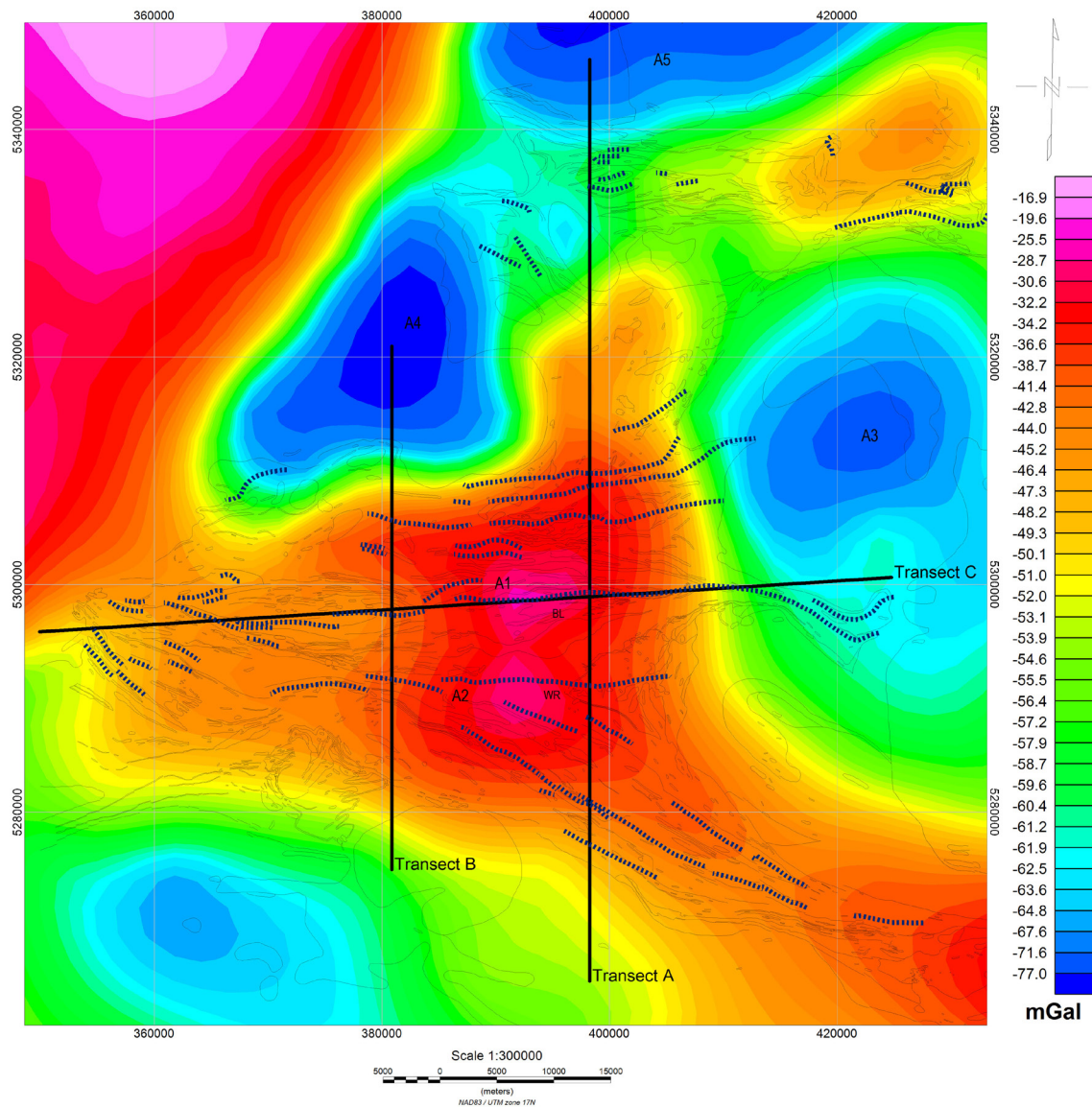
Figure 3. Bouguer anomaly map of the SGB (mGal). Coordinate System NAD-83/ UTM Zone 17 N. The black solid lines indicate the traces of the profiles (transects) along which 2.75D forward modelling was conducted, in order to study the depth and geometry of the geologic bodies and structures of the area. In grey thin lines are represented the geological contacts that occur in the Swayze area (see also the Geological Map in Figure 2). The thick dark blue dashed lines indicate fold axes in the Swayze greenstone belt area. BL and WR correspond to the Brett Lake and the Woman River folds, which are discussed in the text. A1 to A5 indicate the different areas discussed in the Qualitative Analysis section. The Bouguer Anomaly grid file was downloaded from the Geoscience Data Repository of Natural Resources Canada.
