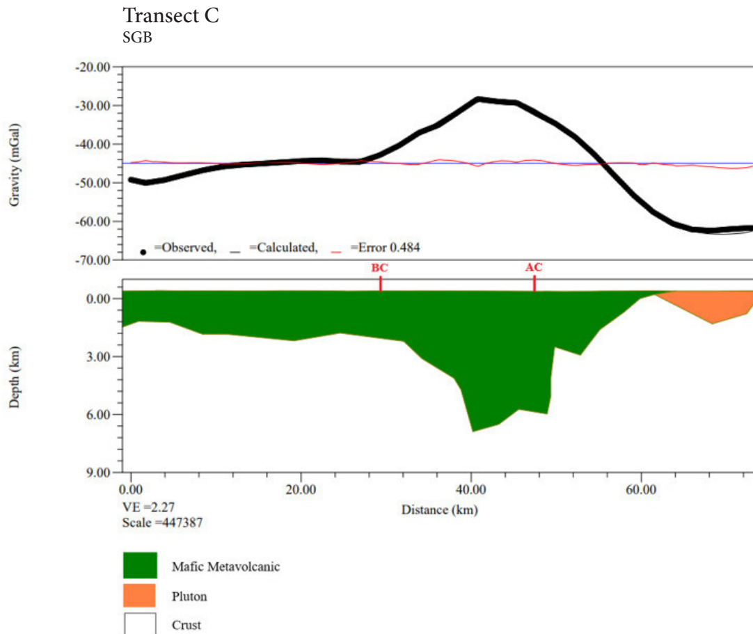
Figure 6. Gravity model along Transect C: Mafic Metavolcanic, \rho=2.89 \text{ g/cm}^3 ; Pluton, \rho=2.66 \text{ g/cm}^3 ; Crust, \rho=2.72 \text{ g/cm}^3 . The two red vertical lines shown at the top of the model panel and labelled AC and BC represent the crossing location between Transect A and Transect C, and between Transect B and Transect C, respectively. The RMS error was of 0.484. The model was obtained with the GM-SYS Extension of the Geosoft – Oasis montaj software.
