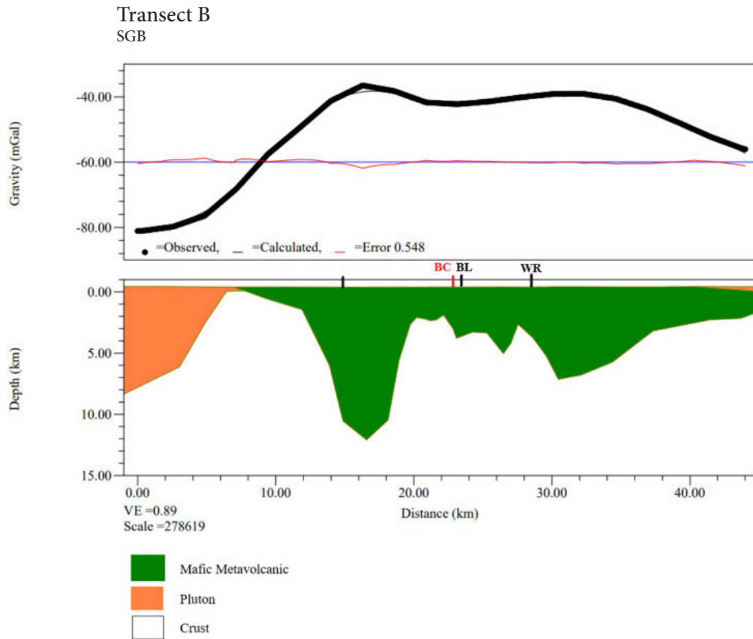
Figure 5. Gravity model along Transect B: Mafic Metavolcanic, \rho=2.89 \text{ g/cm}^3 ; Pluton, \rho=2.66 \text{ g/cm}^3 ; Crust, \rho=2.72 \text{ g/cm}^3 . The black vertical lines shown at the top of the model panel indicate the locations of the different fold axes crossed by the transect. The red vertical line represents the crossing location between Transect B and Transect C. WR-Woman River Anticline, BL-Brett Lake Syncline, BC-Crossing between Transect A and Transect C. The RMS error was of 0.548. The model was obtained with the GM-SYS Extension of the Geosoft – Oasis montaj software.
