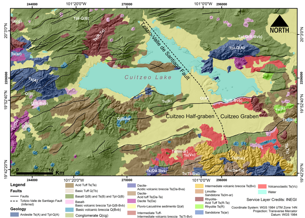
Figure 3. Regional, geologic map of the Morelia-Cuitzeo Lake region showing the Cuitzeo half-graben and graben, separated by the Titzio-Valle de Santiago Fault.
