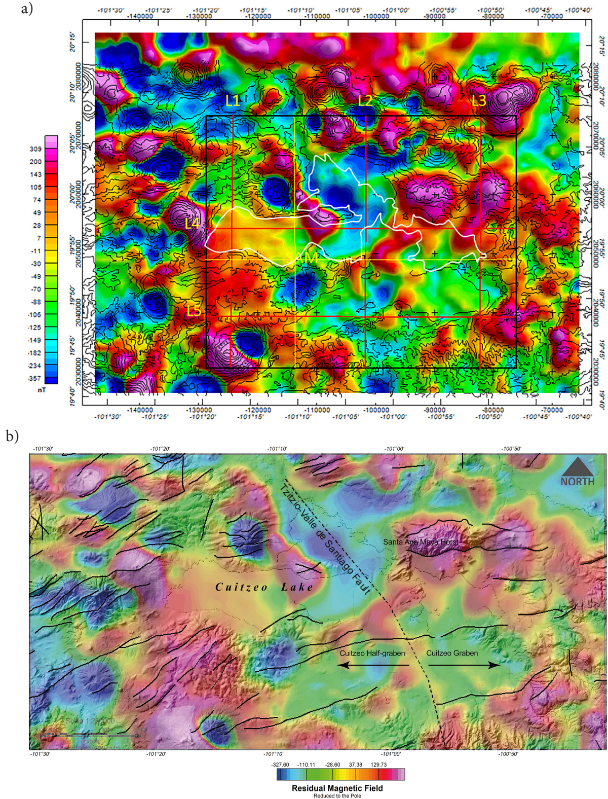
Figure 4. a) Magnetic map reduced to the pole of the Cuitzeo Lake region; elevation contours are shown for correlation, as well as the lake's outline (white). The black rectangle indicates the region in which a 3D inversion of the magnetic field is performed; the red lines (L1-L5) indicate where magnetic susceptibility cross-sections are obtained from such an inversion. SAM, Location of San Agustín del Maíz at the intersection of the two, perpendicular, yellow lines. b) Magnetic map reduced to the pole (Baranod and Naudy, 1964), superposed to the geologic map in Figure 3. Parameter values of the magnetic field: Inclination 47.60^\circ , Declination 7.47^\circ .
