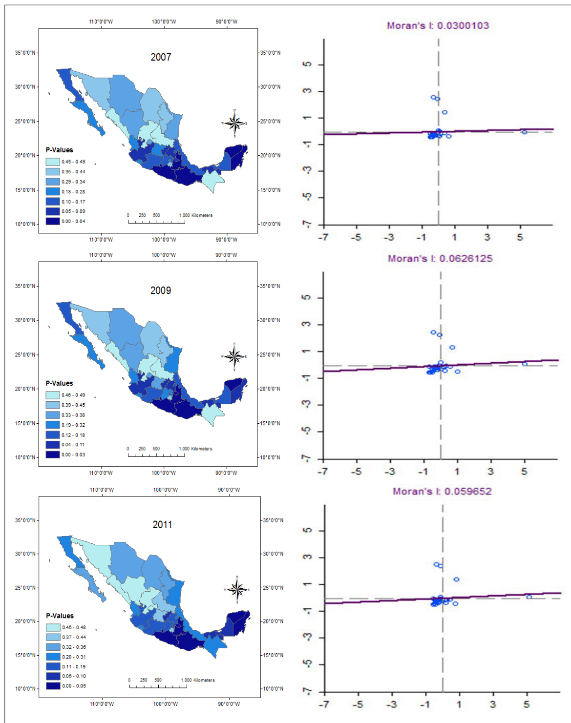
Figure 2: Local Moran's I of Labor Productivity for Selected Years. Source: Institute of Statistic, Geography, and Information (INEGI). Maps and Moran's scatterplots elaborated by the authors using ArcMap and GeoDa, respectively. LISA estimates use the queen criterion of contiguity. Inference is based on 10,000 random permutations
