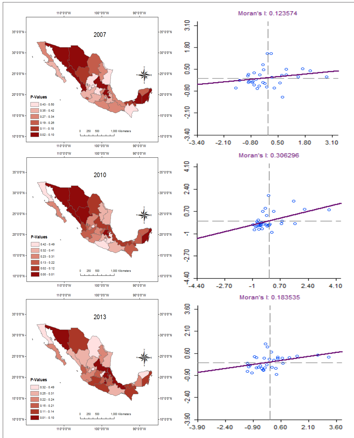
Figure 1: Local Moran's I of Drug-Related Violence (Homicide, Kidnapping, and Extortion) per 100,000 Population for Selected Years. Source: Executive Secretary of the National System for Public Security (SESNSP). Maps and Moran's scatterplots elaborated by the authors using ArcMap and GeoDa, respectively. LISA estimates use the queen criterion of contiguity. Inference is based on 10,000 random permutations.
