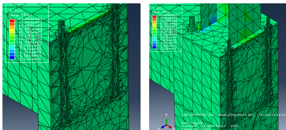
Figure 24. Shear stresses in base plate and anchor bolts. Source: [4]
