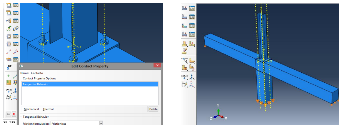
Figure 15. Contact property between surfaces and support conditions for mathematical model. Source: [4]
