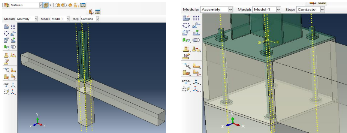
Figure 17. Distribution of materials in the model (Steel in green, concrete in beige). Source: [4]
