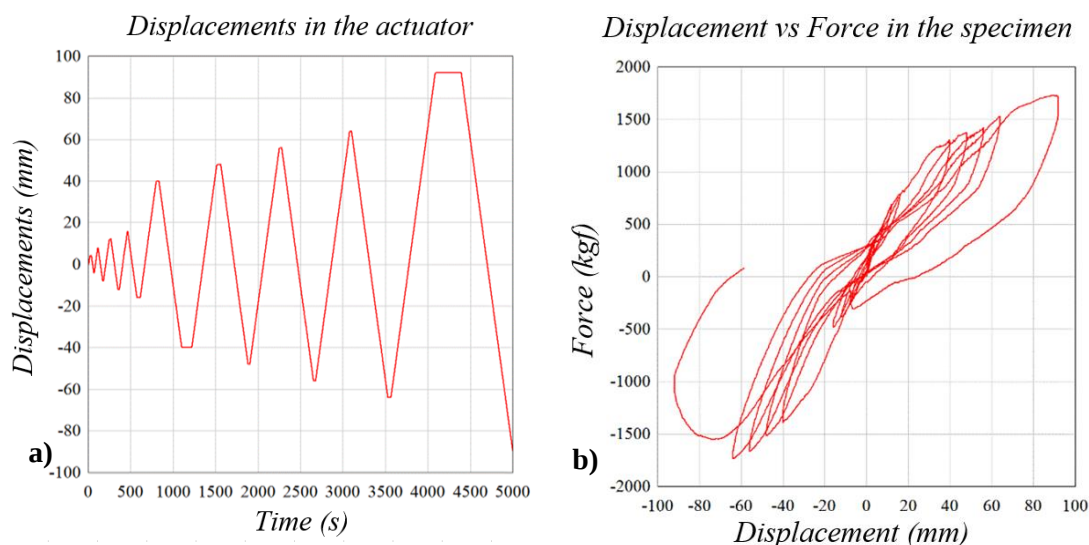
Figure 10. a) Displacement history, b) Concrete cylinders hysteresis. Source: [1]
