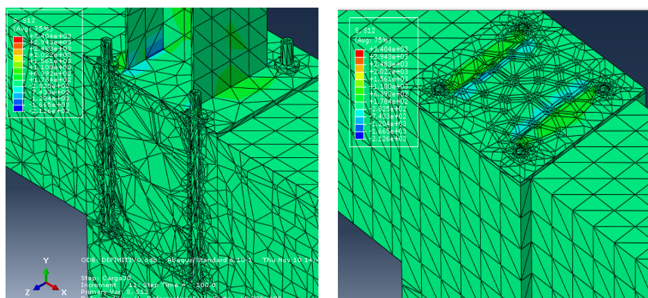
Figure 23. Shear stresses in base plate and anchor bolts. Source: [4]
