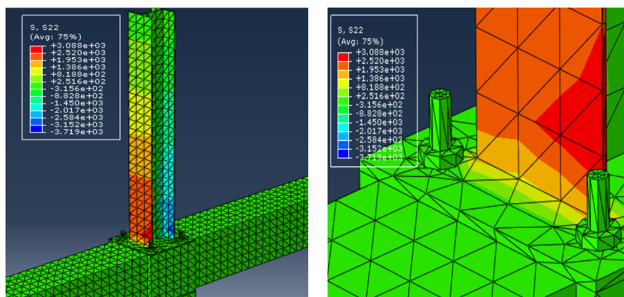
Figure 21. Stresses in the HEA profile. Source: [4]
