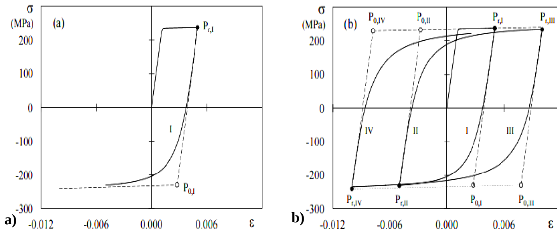
Figure 5. Menegotto and Pinto model. a) First cycle, b) Subsequent. Source: [6]
