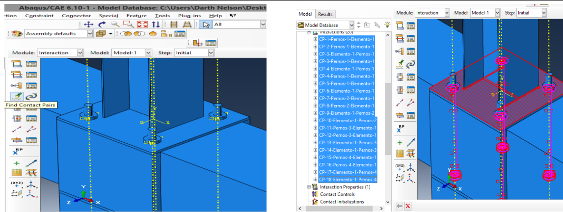
Figure 14. Contact surfaces in the mathematical model. Source: [4]
