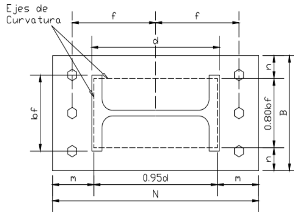
Figure 7. Critical stress zone on the base plate with open core profiles. Source: [12]
