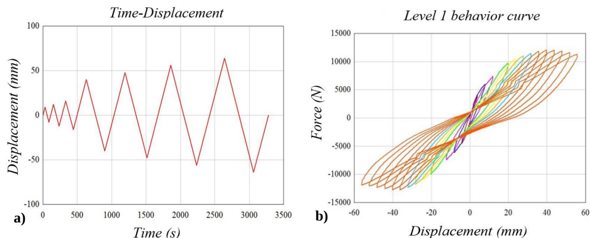
Figure 2. a) A cyclic test example, b) Hysteretic behavior. Source: [1]
