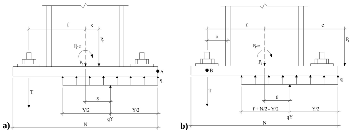
Figure 8. a) Schema of stresses due to small bending moments, b) Large bending moments. Source: [9]
