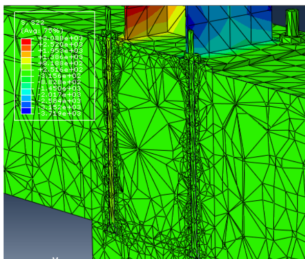
Figure 22. Tensile stress on anchor bolts. Source: [4]
