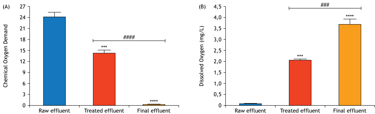
Figure 3. Determination of chemical oxygen demand (A) and dissolved oxygen (B) of pig farming effluent samples before and after TEVAP treatment. The results are the mean of independent experiments ( n = 3 ) performed in triplicate.
