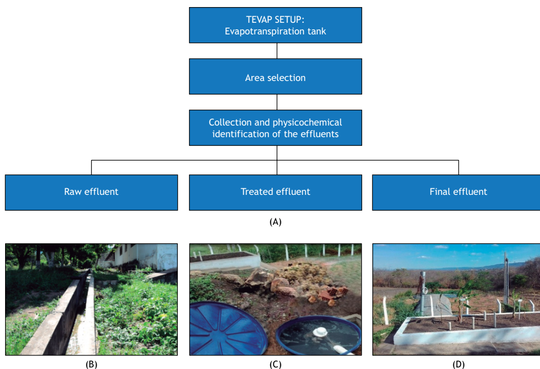
Figure 1. Study development flowchart. Sampling locations are indicated: (A) TEVAP setup flowchart and its respective collection phases for analysis; (B) channel through which the effluent flows after pig pen wash; (C) settling box that temporarily receives pig manure before being stored in the TEVAP; and (D) TEVAP - overlapping culture septic basin, germinated after evapotranspiration.
