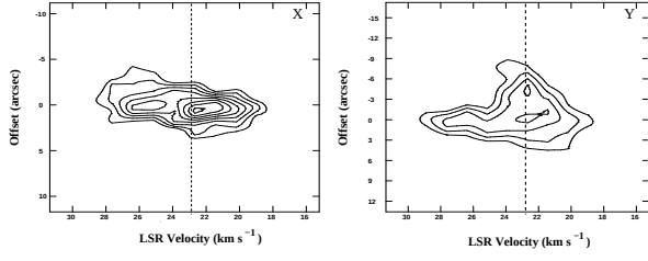
Fig. 7. \text{NH}_3(2,2) position–velocity (PV) diagram of the HMC presented as grey-scale in Figure 6a and 6b. The plots are slices in the directions X and Y shown in the lower-right corner in Figure 6b. The origin of the position axes is located at \alpha_{2000} = 18^{\text{h}}12^{\text{m}}40^{\text{s}} , \delta_{2000} = -18^{\circ}24'15'' . Contours are at -4, 4, 5, 6, 7, 8, 9, 10, 11 \times 1.6 \text{ mJy beam}^{-1} . Dashed lines mark the systemic velocity of the core at \approx 23 \text{ km s}^{-1} .
