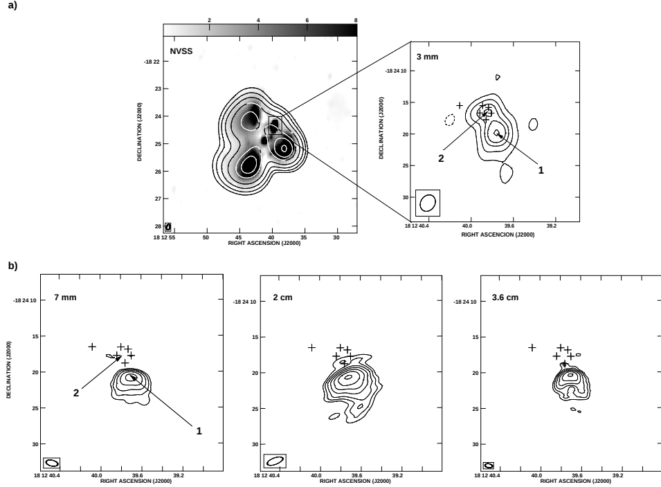
Fig. 1. G12.21-0.10 (G12). a) Left : 21 cm NVSS map (contours) superposed on the 3.6 cm VLA D-configuration image in gray-scale (de la Fuente 2007). The NVSS beam size is 45'' , while that of the 3.6 cm beam, shown in the lower-left corner, is 12''.5 \times 7''.3 at P.A. = -13^\circ . Contours are -3, 3, 6, 12, 24, 48, 68, 96 \times 3 mJy beam ^{-1} . The gray-scale is 0.16 to 8 mJy beam ^{-1} . These maps represent the extended emission in G12. Right : A close up view of the UC component traced by radio continuum emission at 3 mm (see § 2). Contours are at -3, 3, 9, 18, 27, 48 times RMS noise of 1.7 mJy beam ^{-1} . The beam size is shown in the bottom left panel. The positions of the the UC H II region and the molecular clump are labeled as 1 and 2 respectively. In all panels, the crosses mark the position of the water masers from Hofner & Churchwell (1996). b) Radio continuum emission at 0.7, 2, and 3.6 cm (VLA-CnB) toward G12. The contour levels correspond to -1, 1, 2, 4, 8, 16, 32, 64 \times RMS noise presented in Table 3 for each wavelength. The synthesized beam for each map is shown in the lower left corner (see Table 3).
