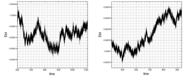
Fig. 5. Total energy as a function of time for Models 1A (left) and 1B (right) over the entire orbit integration interval of 85 t_{cross} . The total energy fractional errors ( E_{fe} ) are 3 \times 10^{-7} (left) and 4 \times 10^{-6} (right). The vertical axis on both graphs spans an energy interval of 0.0000012 units.
