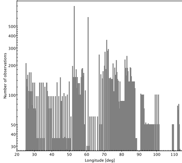
Fig. 1. Number of observations for each observing window corresponding to objects in the interval 8.6^\circ \text{W} < \lambda^\circ < 117.5^\circ \text{W} and -0.165 < \delta^\circ < 0.165 . The available number of observations allows the determination of the relative motion of orbiters in the GEO ring over different time scales.
