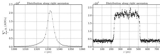
Fig. 5. Distribution of the signal along the \alpha ( x ) coordinate. Left panel shows a point source PSF. Right panel shows a streak represented as a tepui.
