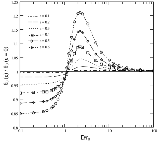
Fig. 1. Normalized FWHMs of a perfect telescope with annular aperture for different D/r_0 ratios (horizontal axis is in logarithmic scale).
