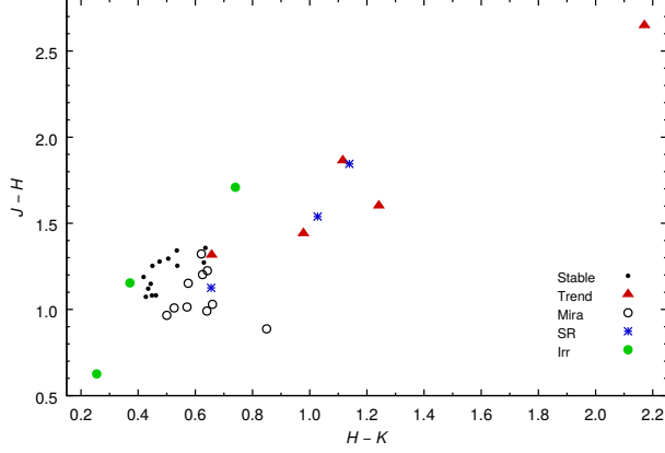
Fig. 8. The J-H , H-K diagram of our variables. The carbon star #234 is located at the upper-right corner; the main sequence star #303 is at the lower left corner. Variability type is coded as follows: open circles = Mira; blue stars = semiregular variables; filled red triangles = stars with a long term trend; filled green circles = irregular variables; dots = non-variable (stable) stars. The color figure can be viewed online.
