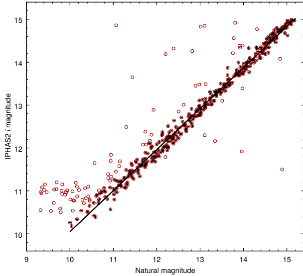
Fig. 1. Comparison of our “ natural magnitudes” and IPHAS2 i magnitudes for our non-variable red stars (open circles) in the field of \gamma Cas. Black stars are used to compute the linear correlation described in the text. The color figure can be viewed online.
