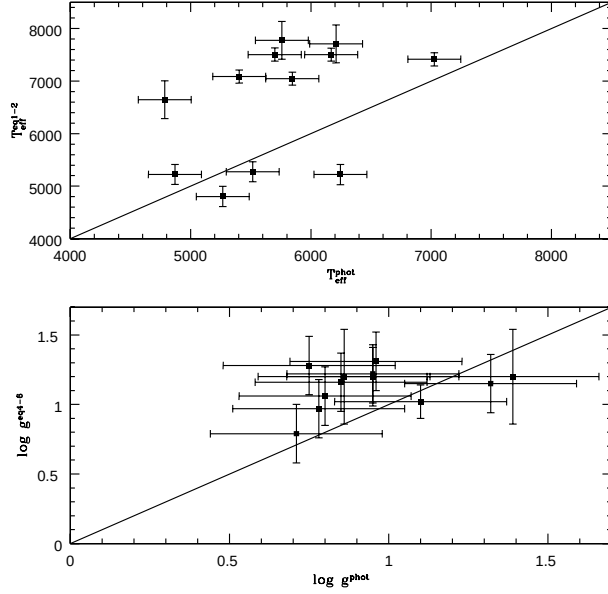
Fig. 5. Comparison between effective temperature and surface gravity obtained from 2MASS photometry by Molina (2012) and effective temperature and surface gravity estimated in this work (see upper and bottom panels). The solid straight line in each panel denotes perfect agreement between the sets of data.
