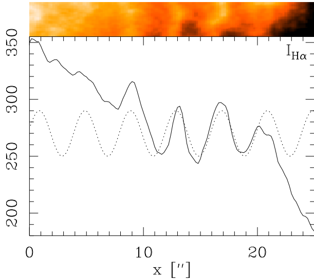
Fig. 3. Top frame: H\alpha emission of the region with the wave-like structure in the SW of the “hill” (corresponding to the box shown in the top frame of Figure 2). Bottom frame: H\alpha emission (in arbitrary units) integrated over the N/S axis of the top box, shown as a function of distance from the E edge of the box (solid line). A sinusoidal curve with a spatial wavelength of 4'' (1600 AU) is also shown (dashed line). The color figure can be viewed online.
