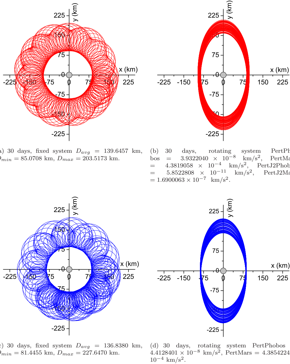
Fig. 7. Trajectories considering an elliptical orbit for Phobos and flat bodies for Mars and Phobos (red) and considering a circular orbit for Phobos and spherical bodies for Mars and Phobos (blue). Phobos initially at apoapsis, D = 85 km, v_x = 0 , v_y = -0.02 km/s, T = 30 days. The color figure can be viewed online.
