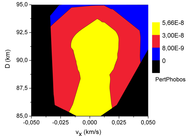
Fig. 3. Integral over time of the force arising from Phobos, in km/s 2 , as a function of D (km) and v_x (km/s). The color figure can be viewed online.
